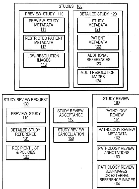
DATA STRUCTURES IN THE EXCHANGE OF STUDIES
