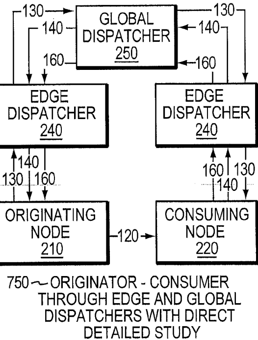
EXAMPLES OF MESSAGE ROUTING PATHS
