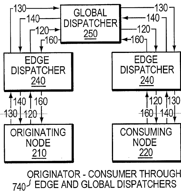
EXAMPLES OF MESSAGE ROUTING PATHS
