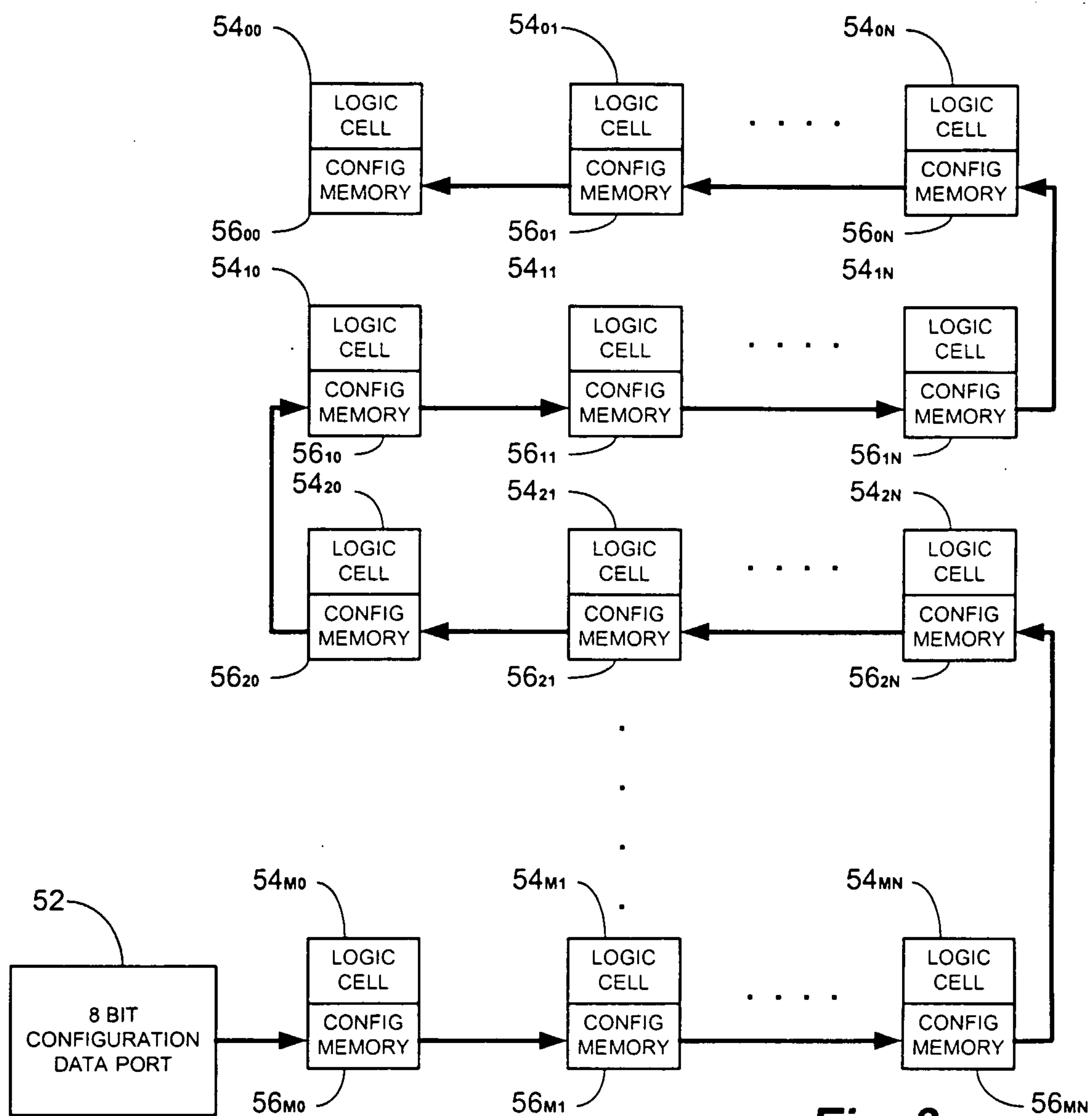
Fig. 3 Prior Art
