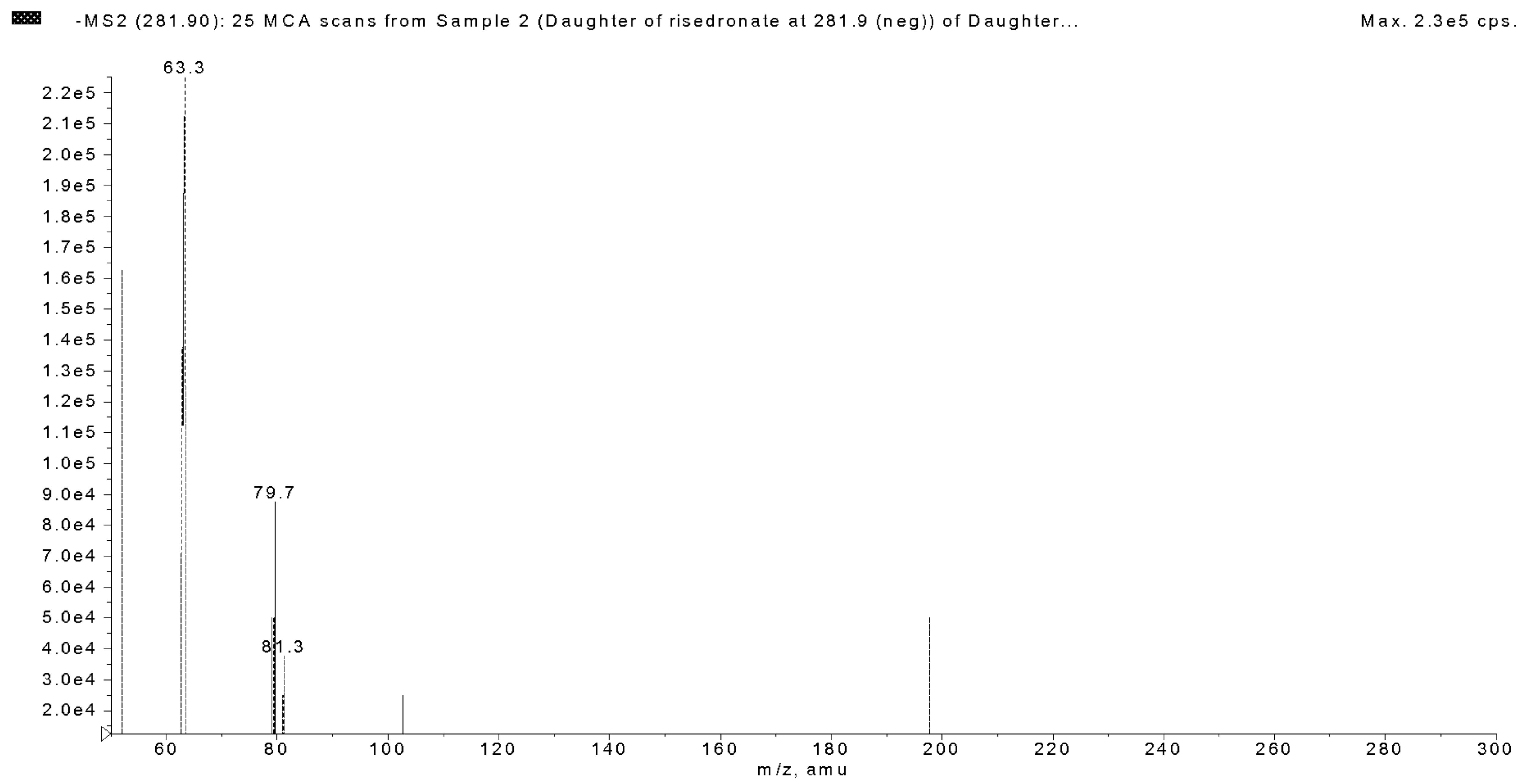
FIGURE 1. ESI-MS Spectrum of Risedronate
