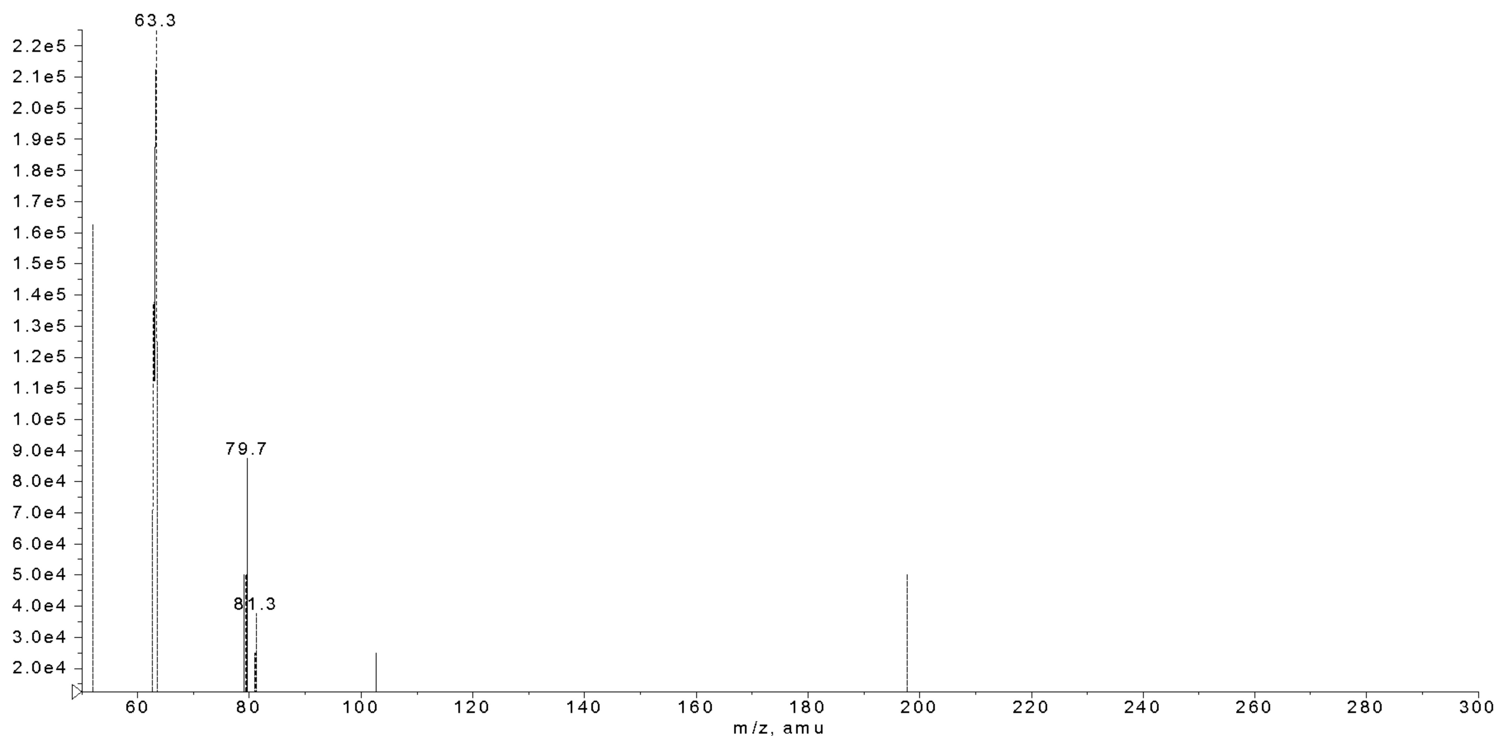
ESI-MS Spectrum of Risedronate
