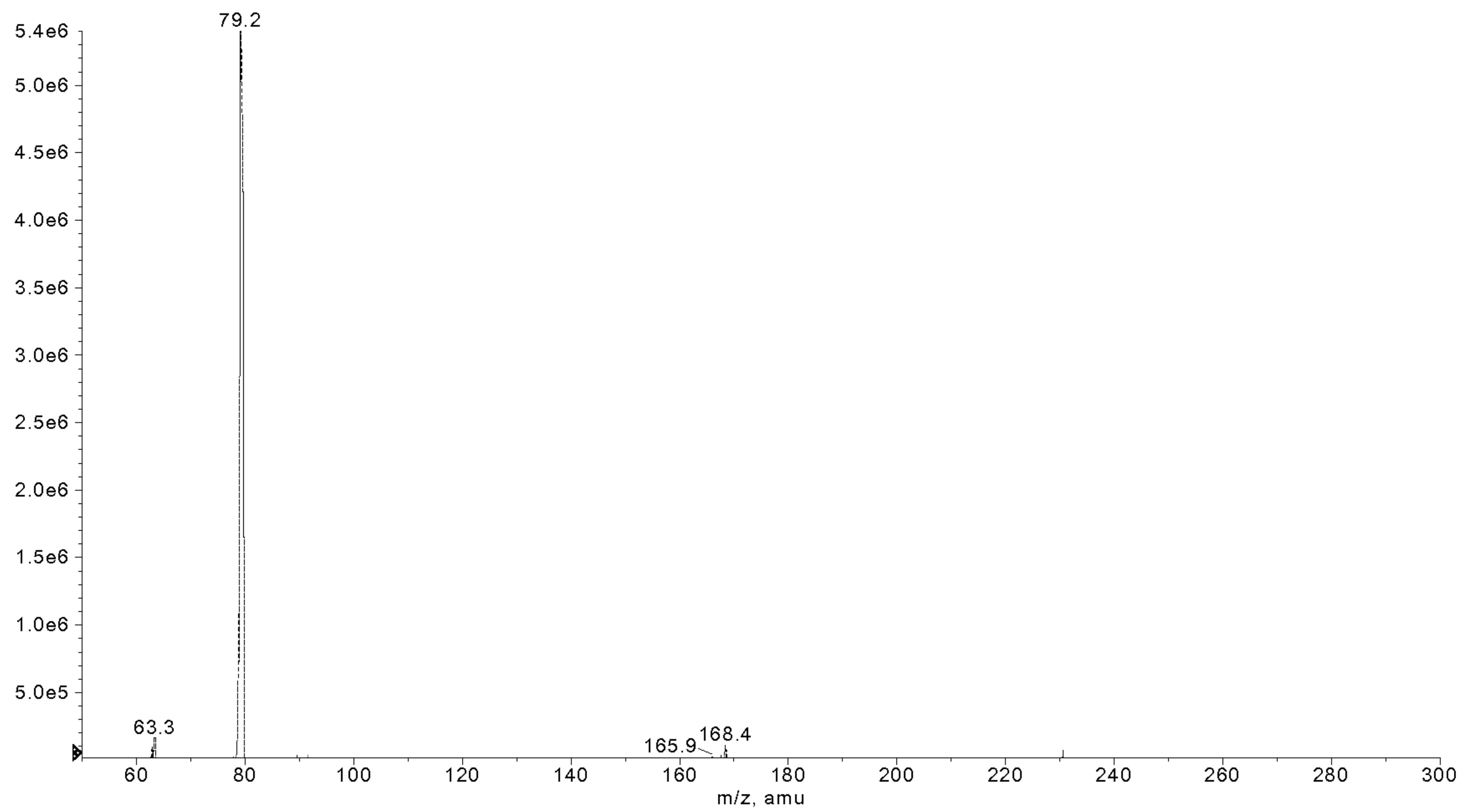
FIGURE 2. ESI-MS Spectrum of Deoxy-Risedronate
