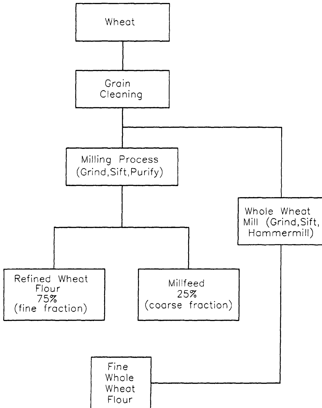
Traditional Mill Process Flow Diagram
