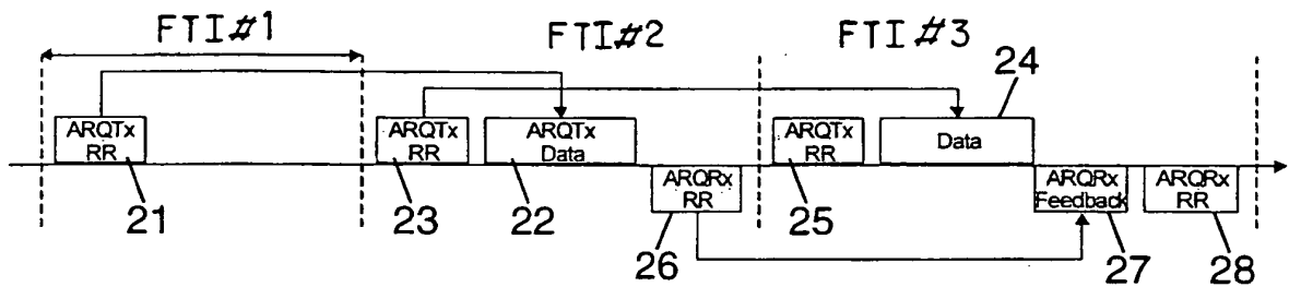
FIG. 2 (PRIOR ART)
