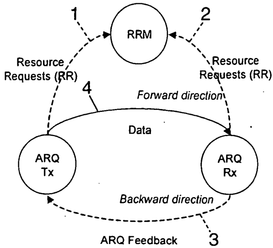
FIG. 1 (PRIOR ART)
