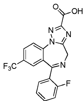
(Compound 1);
