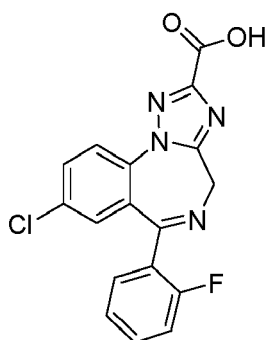
(Compound 1).
