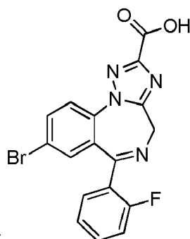
(Compound 4);
