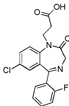
(Compound 16); and
