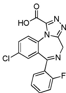
(Compound 15);
