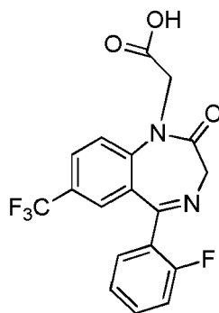
(Compound 15);
