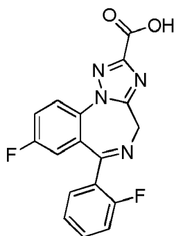
(Compound 3);
