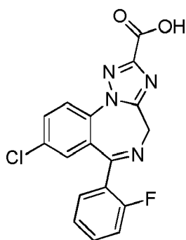
(Compound 1);
