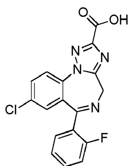
(Compound 1);
