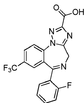
(Compound 1);
