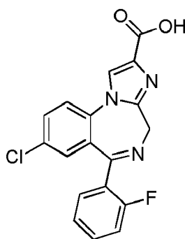
(Compound 12).
