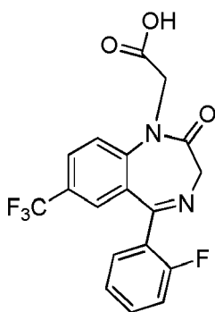
(Compound 16); and
