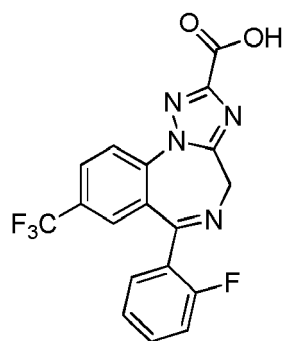
(Compound 1);
