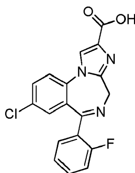
(Compound 11);
