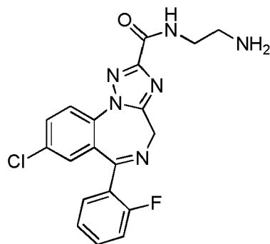
(Compound 9);
