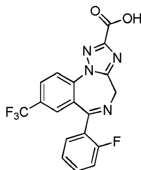
(Compound 1);
