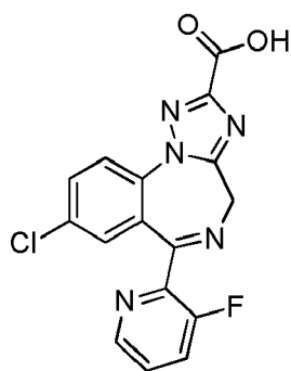
(Compound 11);
