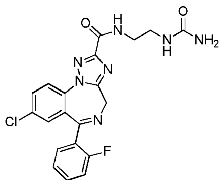
(Compound 5);
