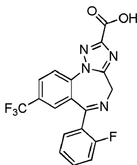
(Compound 2).
