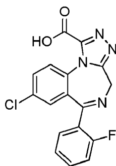
(Compound 15);
