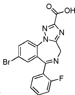
(Compound 4);
