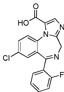
(Compound 13);
