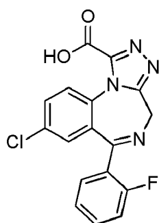
(Compound 15).
