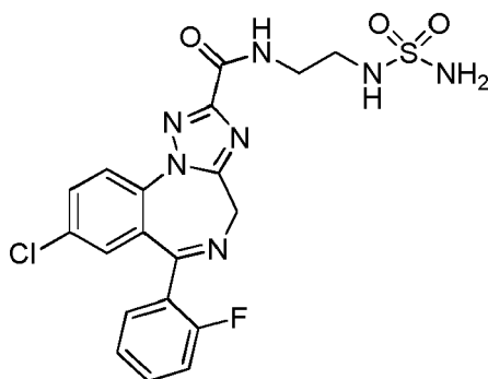
(Compound 9).
