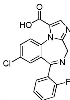
(Compound 14); and
