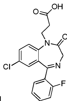
(Compound 17).
