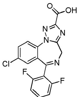
(Compound 5).
