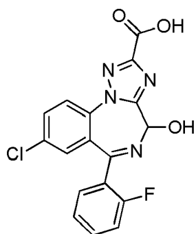
(Compound 13);
