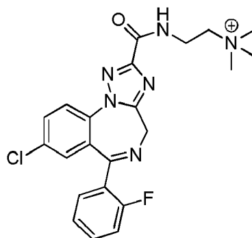
(Compound 7);
