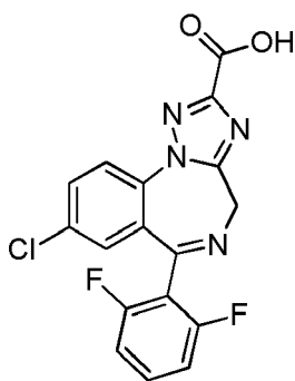
(Compound 5);
