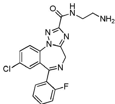
(Compound 10).
