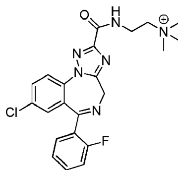
(Compound 7);
