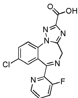
(Compound 11);
