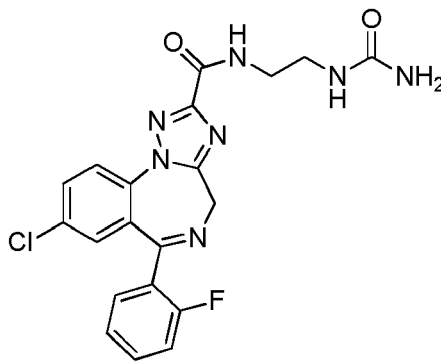
(Compound 5);
