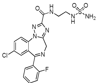
(Compound 9);
