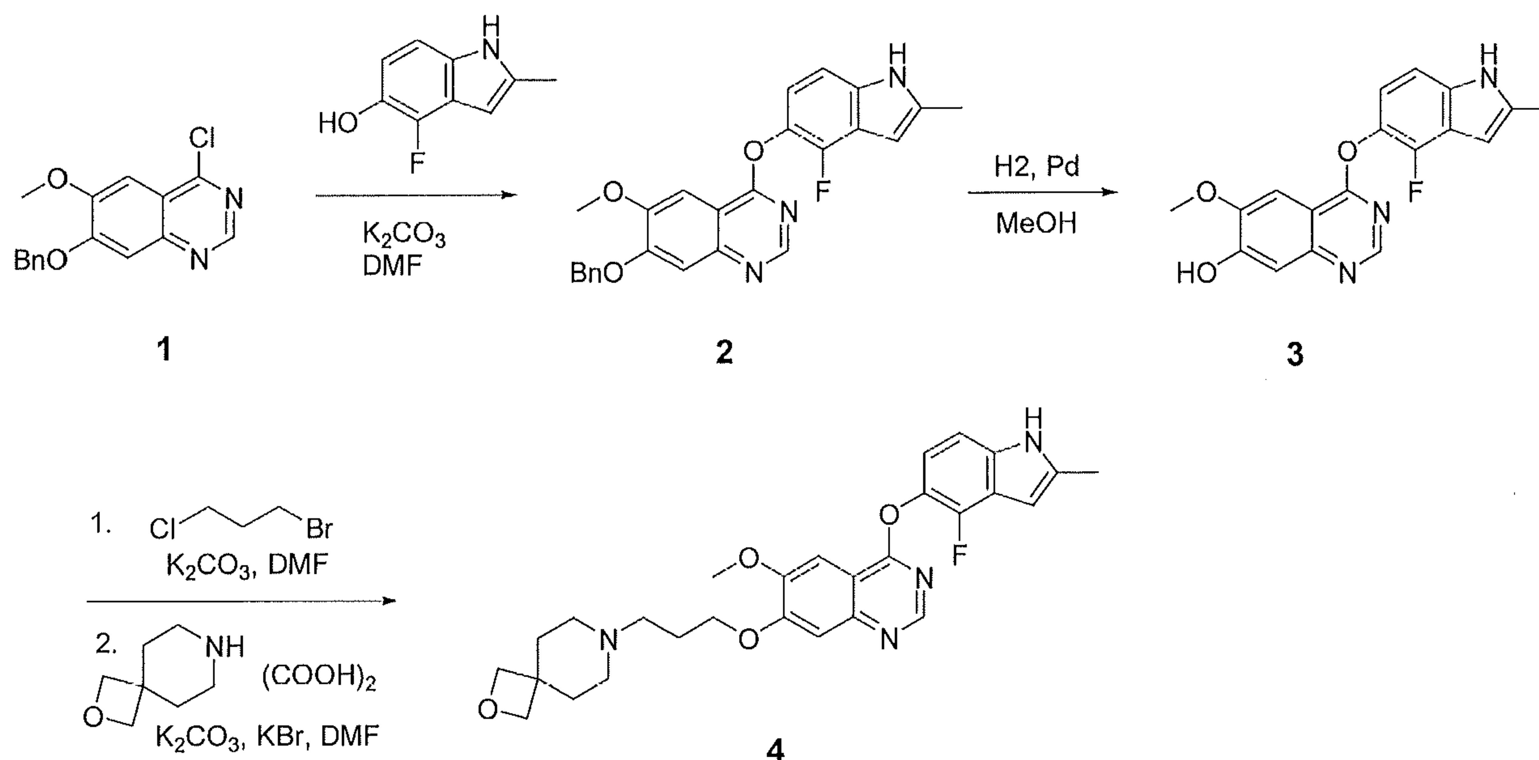
Scheme 1
