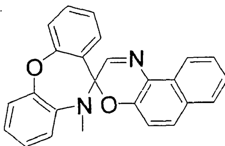
Spirooxazine (1)
