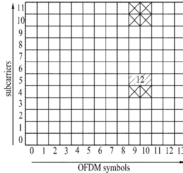
(d) Cell-B (2 Tx) 2Tx CSI-RS pattern for Cell-B: 12 8Tx CSI-RS pattern muted in Cell-B: 1
