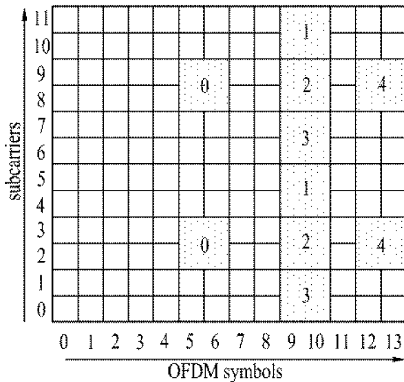
(b) CSI-RS pattern for muting (defined for 8 CSI-RS)
