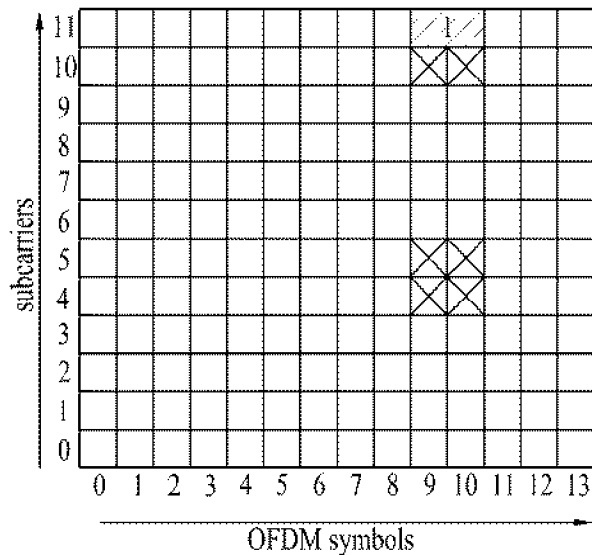
(c) Cell-A (2 Tx) 2Tx CSI-RS pattern for Cell-A: 1 8Tx CSI-RS pattern muted in Cell-A: 1
