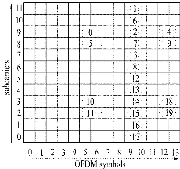
(a) CSI-RC pattern (defined for 2 CSI-RS)
