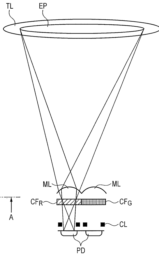
A-A CROSS-SECTIONAL VIEW
