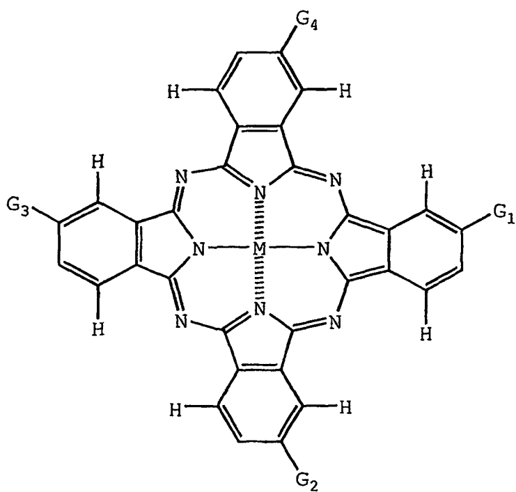
Formula (a)-3:
