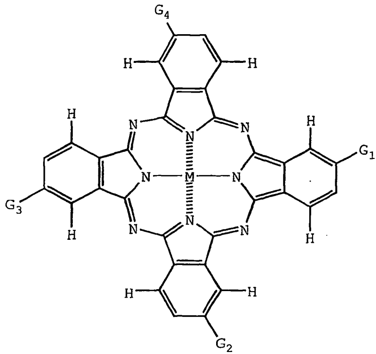
Formula (a)-1:
