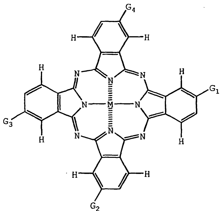
Formula (a)-4:
