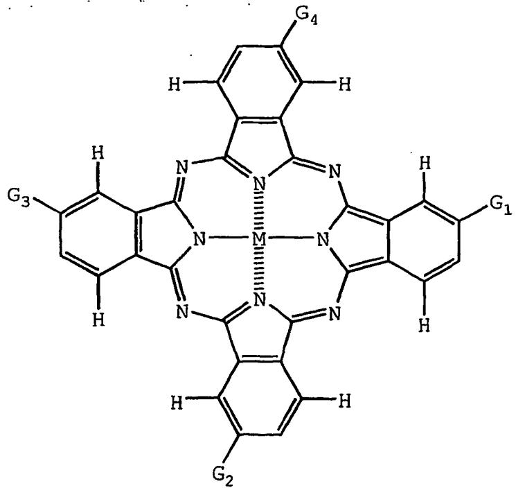
Formula (a)-2:
