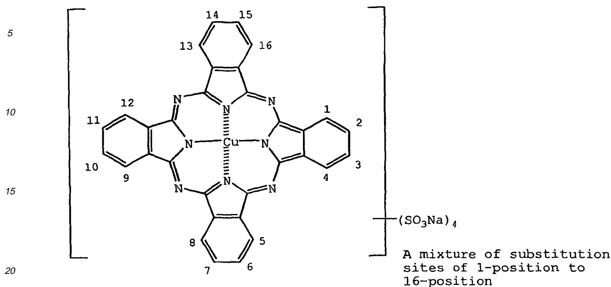
Comparative Compound 1
