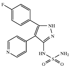
[4-(4-fluorophenyl)-5-(4-pyridinyl)-1H-pyrazol-3-yl] sulfamide
