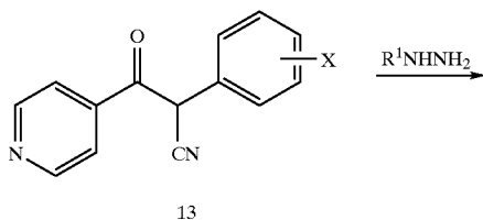
Scheme III
