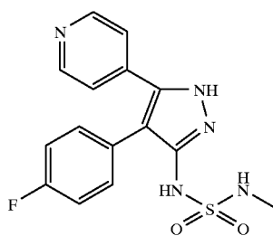
N-[4-(4-fluorophenyl)-5-(4-pyridinyl)-1H-pyrazol-3-yl]-N'-methylsulfamide
