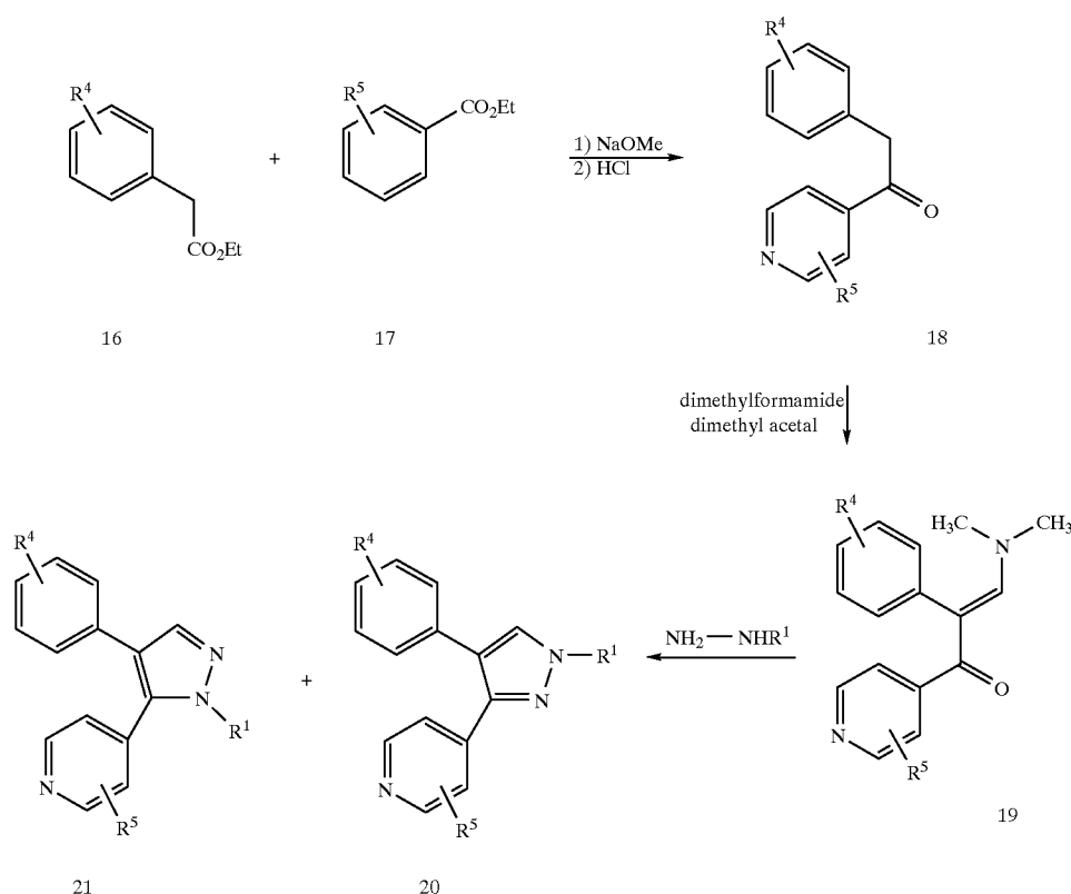
Scheme IV
