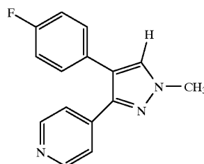
4-[4-(4-fluorophenyl)-1-methyl-1H-pyrazol-3-yl]pyridine
