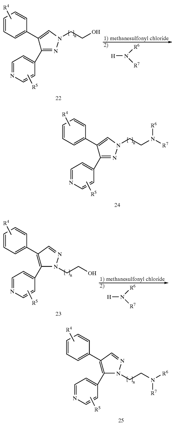
Scheme V
