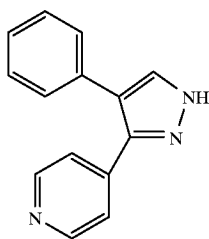
4-(4-phenyl-1H-pyrazol-5-yl)pyridine
