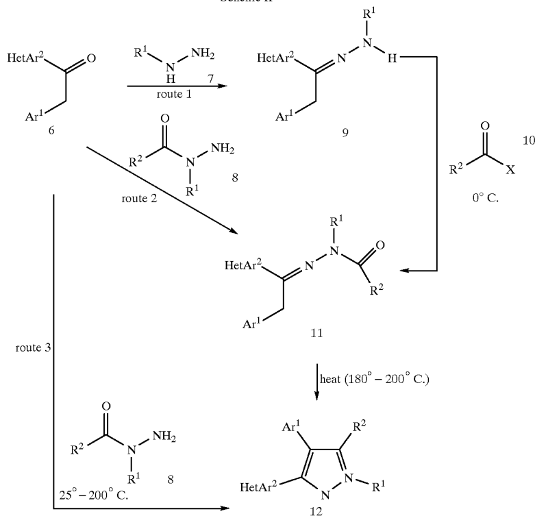
Scheme II
