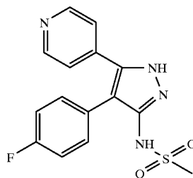
N-[4-(4-fluorophenyl)-5-(4-pyridinyl)-1H-pyrazol-3-yl]methanesulfonamide
