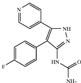
[4-(4-fluorophenyl)-5-(4-pyridinyl)-1H-pyrazol-3-yl] urea
