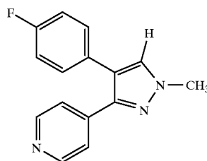
4-[4-(4-fluorophenyl)-1-methyl-1H-pyrazol-3-yl]pyridine
