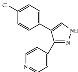
4-[4-(4-chlorophenyl)-1H-pyrazol-3-yl]pyridine
