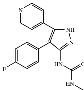
N-[4-(4-fluorophenyl)-5-(4-pyridinyl)-1H-pyrazol-3- yl]-N'-methylurea
