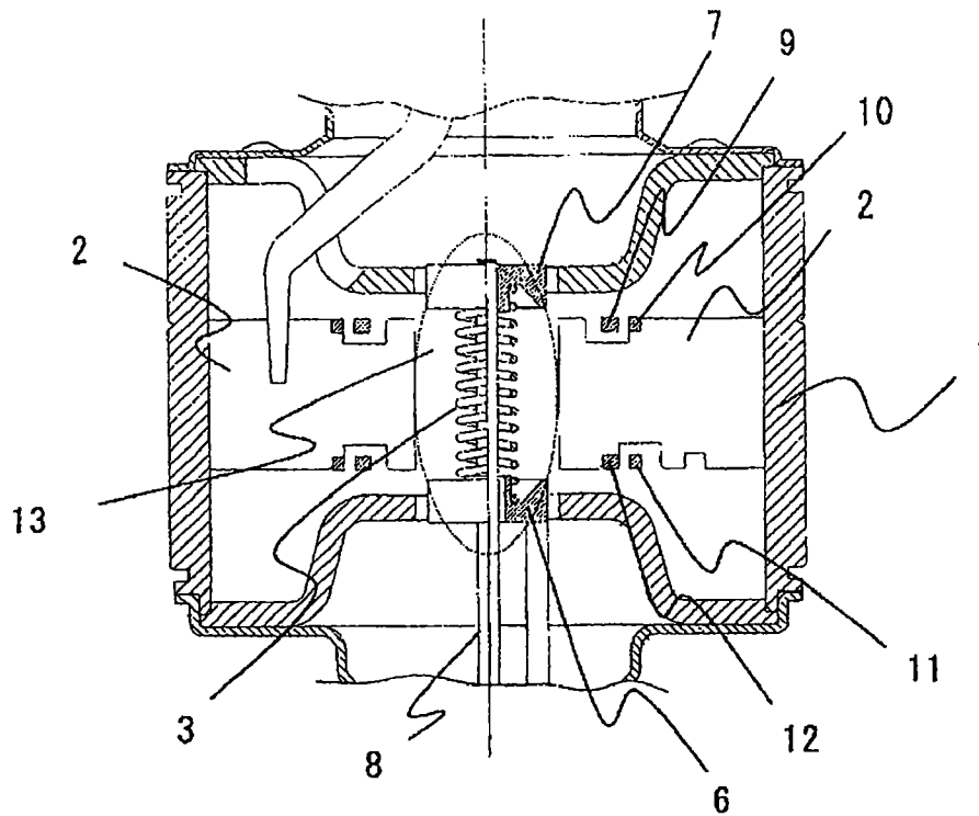
FIG. 33 Prior Art
