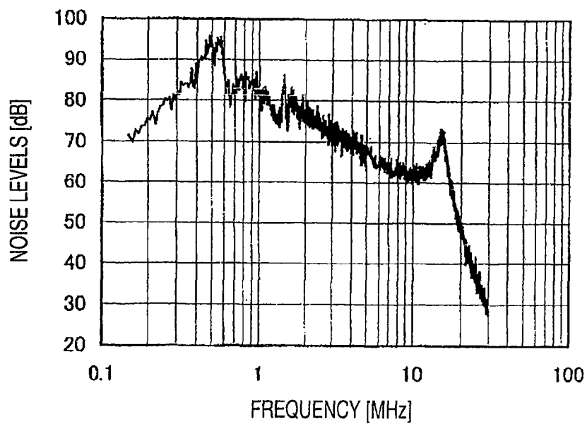
FIG. 35 Prior Art
