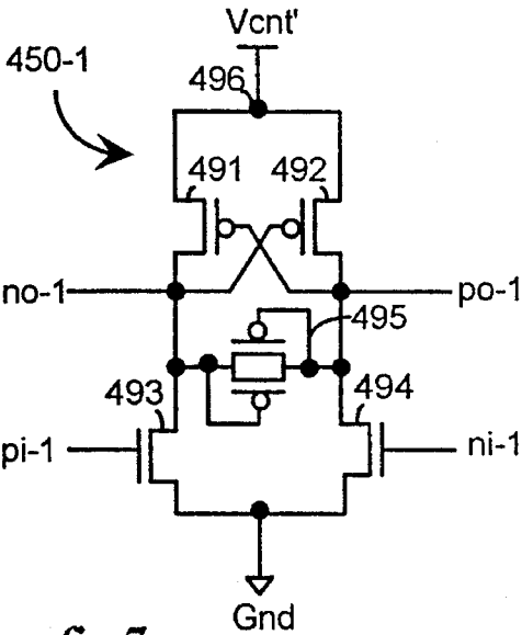
fig.7 prior art
