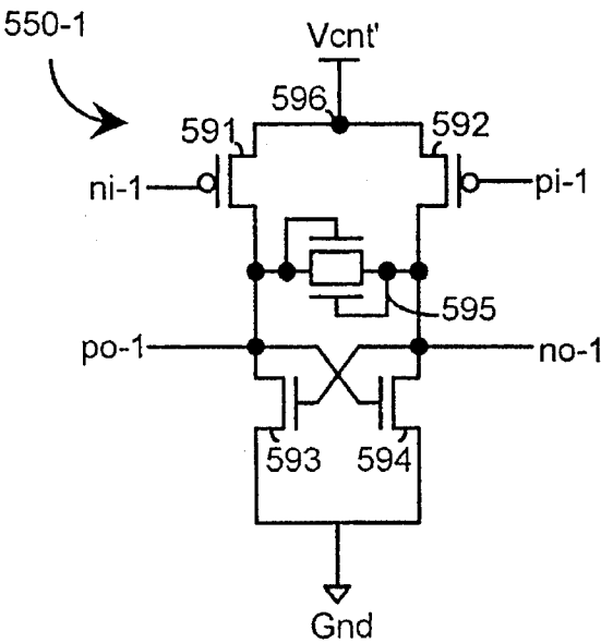
fig.8 prior art
