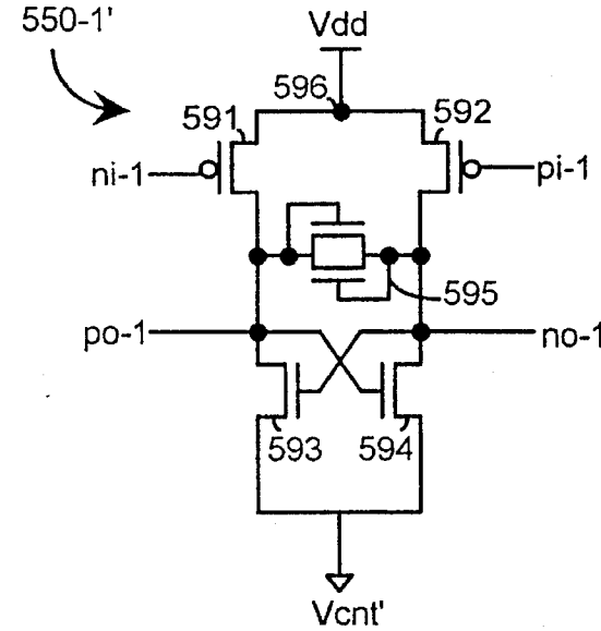
fig.10 prior art
