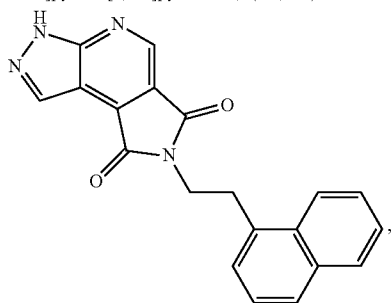
7-[2-(1-naphthyl)ethyl]pyrazolo[3,4-b]pyrrolo[3,4-d]pyridine-6,8(3H, 7H)-dione
