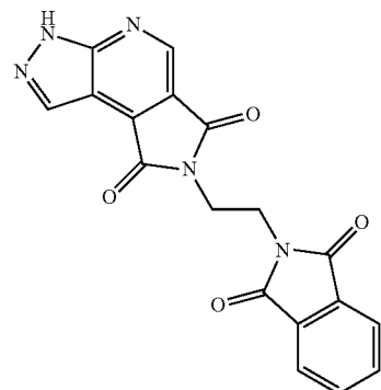
7-[2-(1,3-dioxo-1,3-dihydro-2H-isoindol-2-yl)ethyl]pyrazolo[3,4-b]pyrrolo[3,4-d]pyridine-6,8(3H, 7H)-dione
