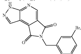
7-(3-bromobenzyl)pyrazolo[3,4-b]pyrrolo[3,4-d]pyridine-6,8(3H, 7H)-dione
