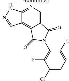
7-(3-chloro-2,6-difluorobenzyl)pyrazolo[3,4-b]pyrrolo[3,4-d]pyridine-6,8(3H, 7H)-dione
