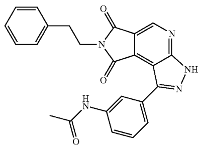
N-[3-[6,8-dioxo-7-(2-phenylethyl)-3,6,7,8-tetrahydropyrazolo[3,4-b]pyrrolo[3,4-d]pyridin-1-yl]phenyl]acetamide
