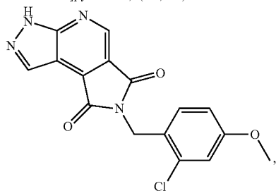
7-(2-chloro-4-methoxybenzyl)pyrazolo[3,4-b]pyrrolo[3,4-d]pyridine-6,8(3H, 7H)-dione
