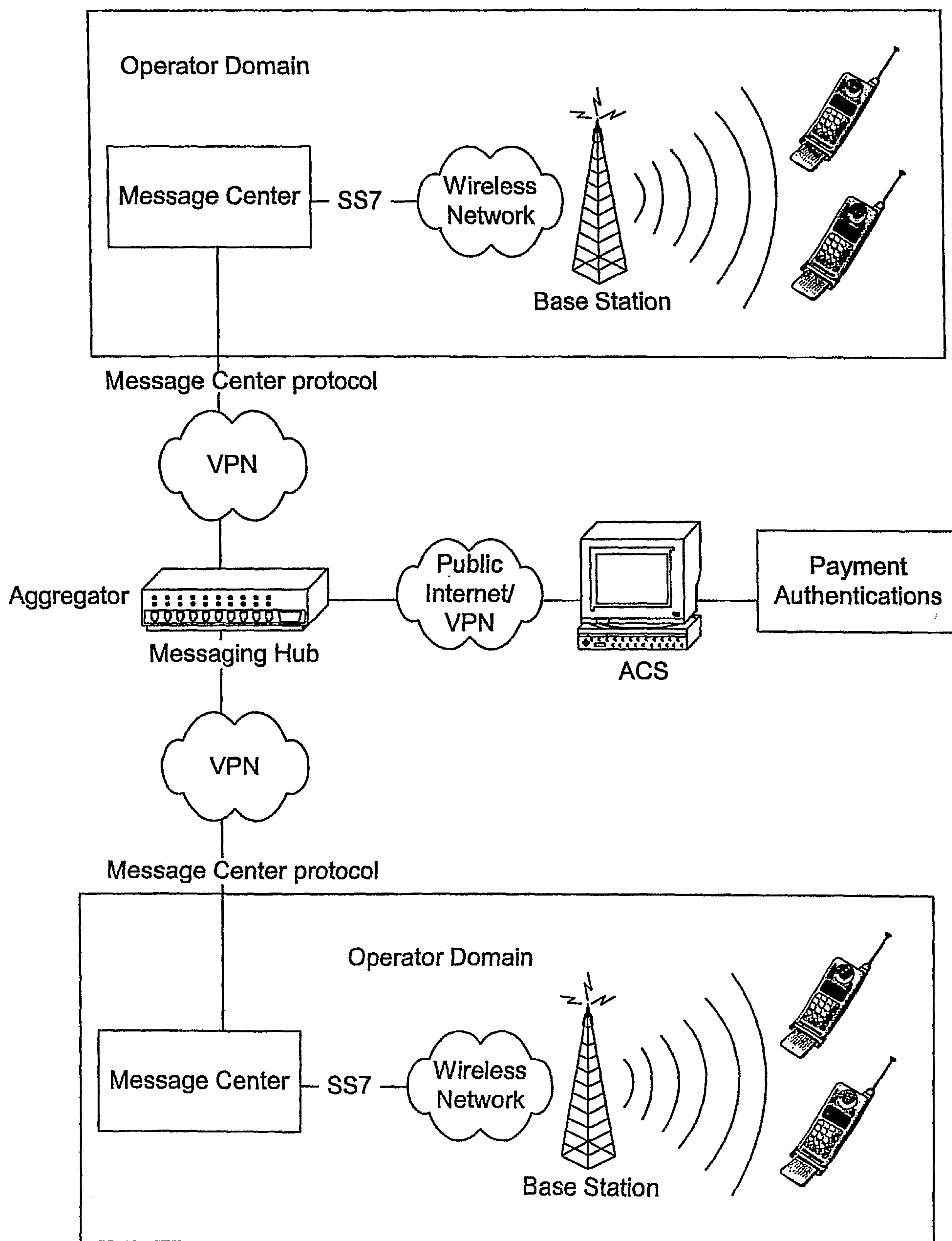
FIG. 15 Two-Way Messaging System
