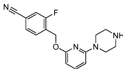
Intermediate 13
