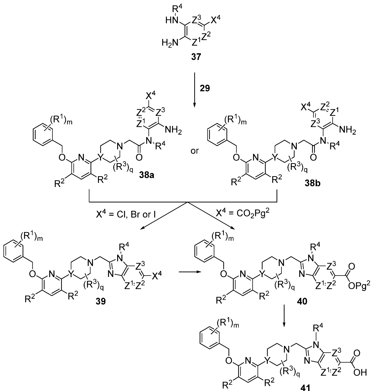
Scheme 9
