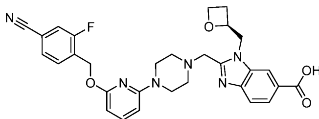
Example 5A-01
