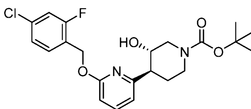
Intermediate 8
