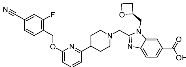
Example 4A-01
