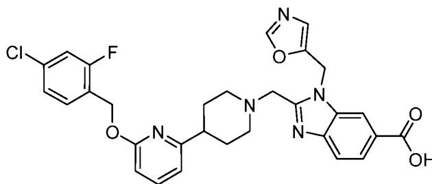
Example 10A-01
