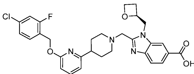
Example 3A-01
