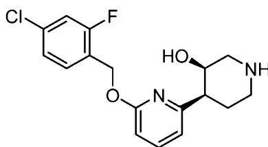
Intermediate 11
