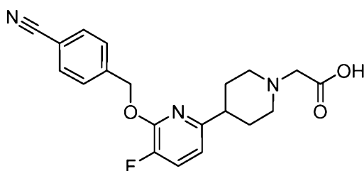
Intermediate 7
