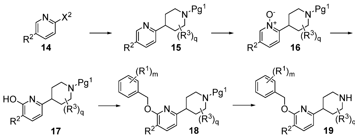
Scheme 5
