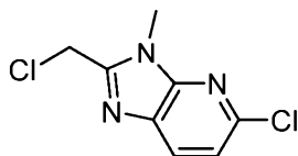
Intermediate 33
