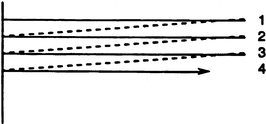
STANDARD CRT RASTER SCAN
