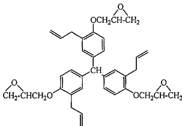
i-6: Compound E obtained in Comparative Example 1
