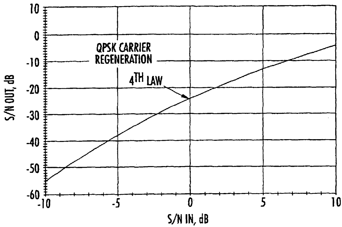
FIGURE 5 (Prior Art)
