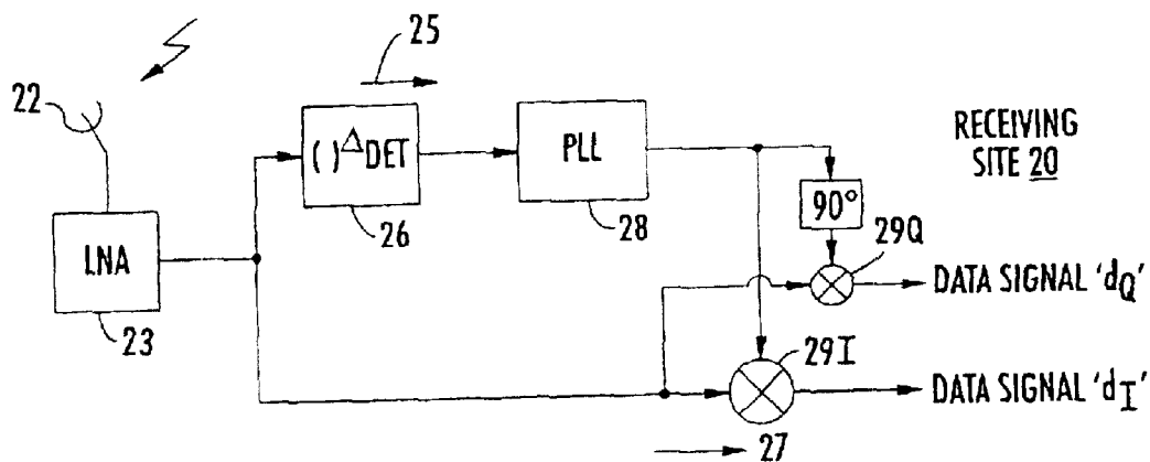
FIGURE 3 (Prior Art)
