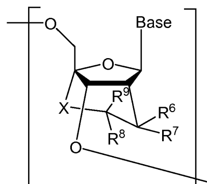
[Chemical Formula 9]
