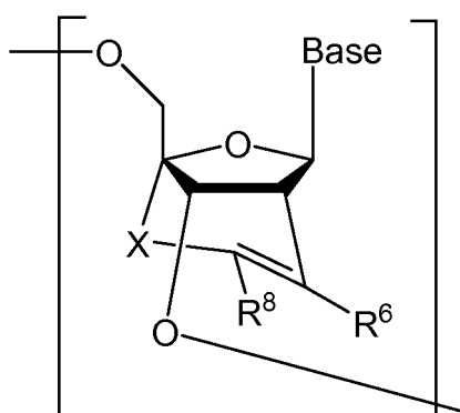
[Chemical Formula 10]
