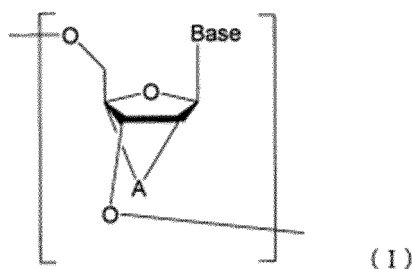
[Chemical Formula 1]
