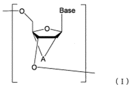
[Chemical Formula 4]
