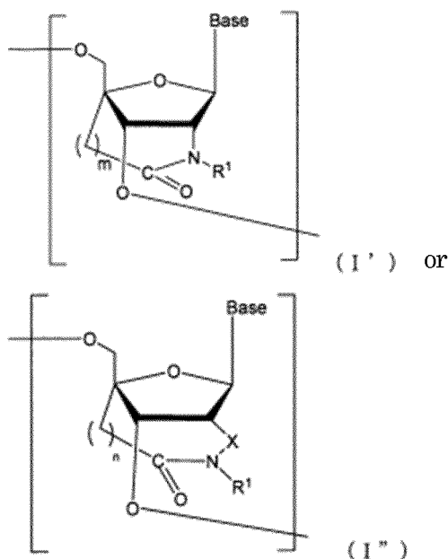
[Chemical Formula 3]
