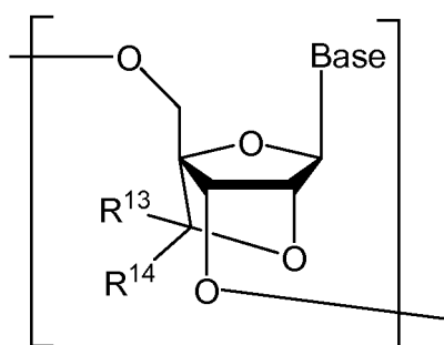
[Chemical Formula 11]
