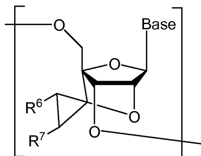
[Chemical Formula 7]
