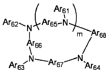
General formula [17]
