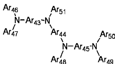
General formula [15]
