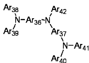
General formula [14]
