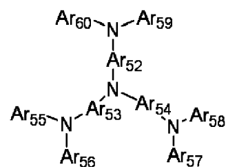
General formula [16]
