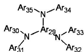
General formula [13]
