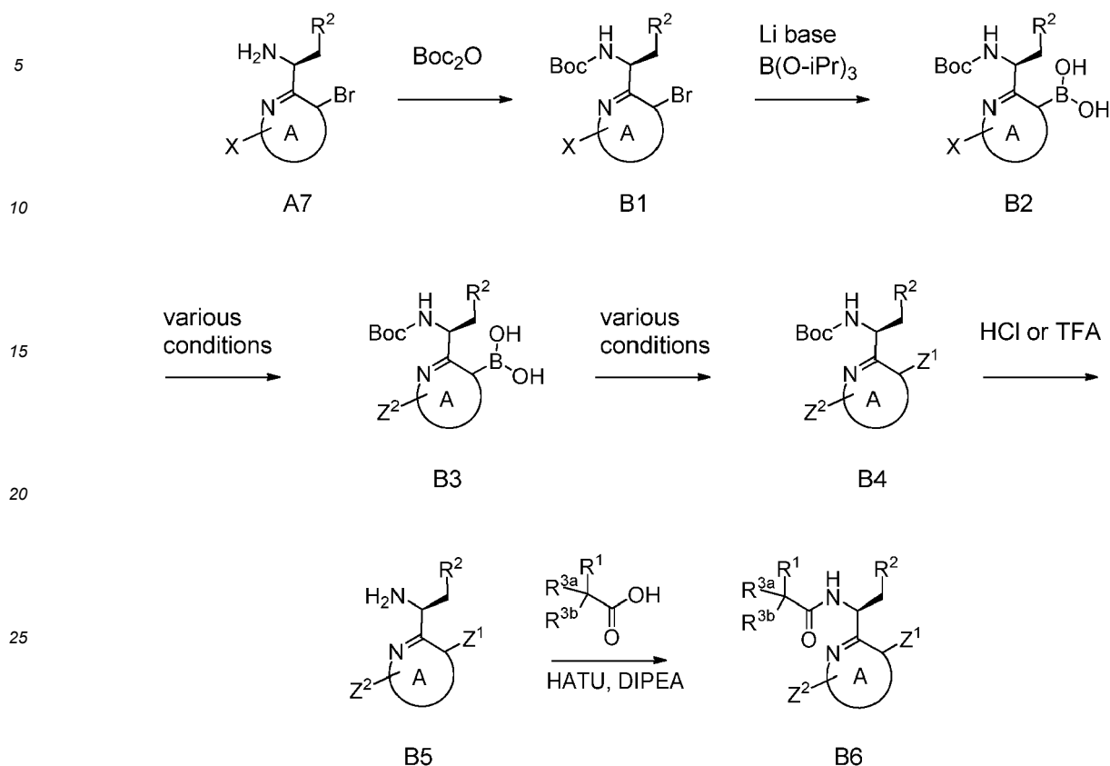
Scheme 2
