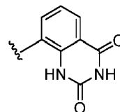
2,4-dioxo-1,2,3,4-tetrahydroquinazolin-8-yl
