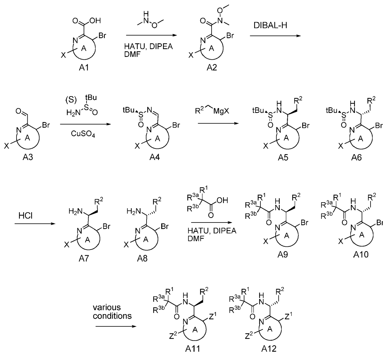
Scheme 1
