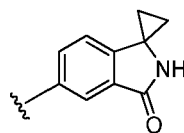
3-oxospiro[cyclopropane-1,1'-isoindolin]-5-yl
