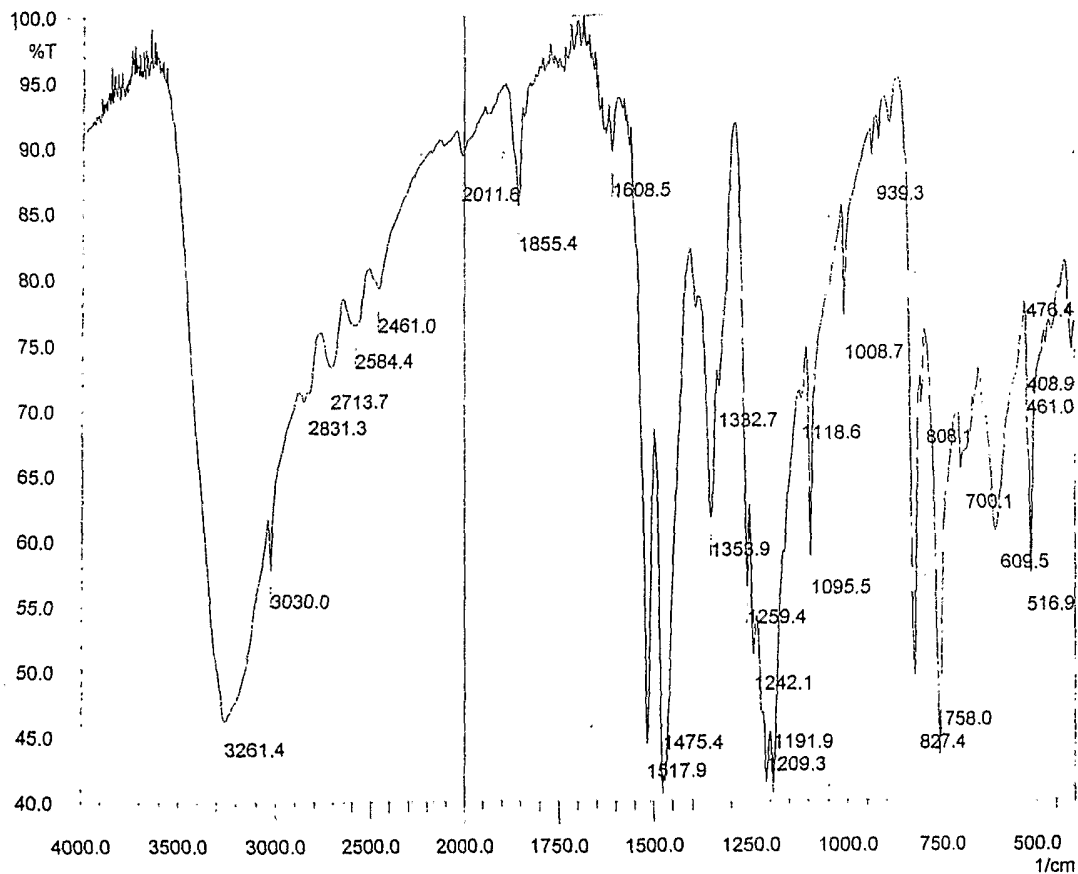
Fig 22. FTIR spectroscopic profile of hydroquinone.
