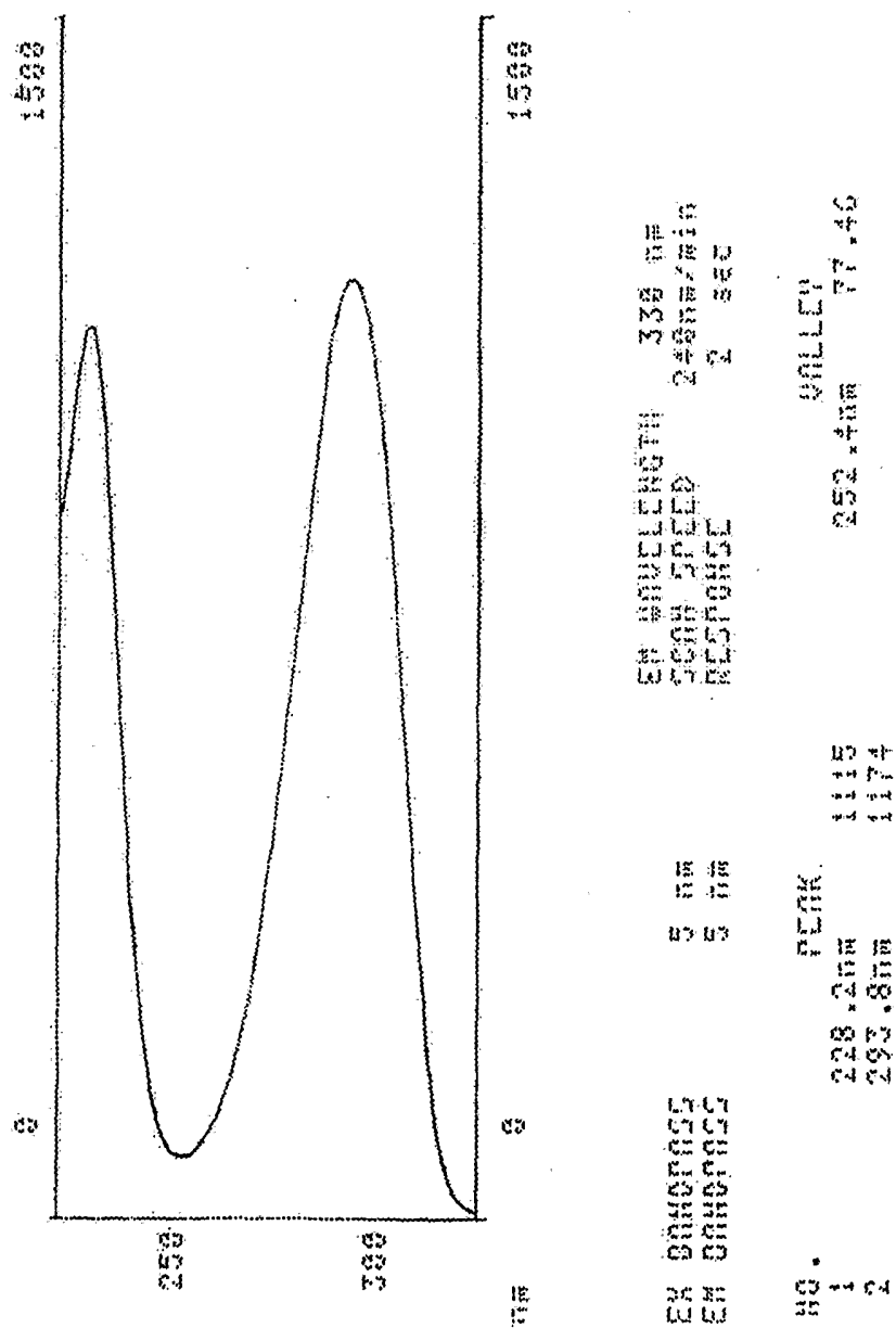
Fig 7a. Fluorescence spectroscopic profile of the cs-oxidant in methanol. The emission was at 330 nm and the excitation scanning was measured from 220 nm to 325 nm. The excitation maxima were at 228.2 nm and at 293.8 nm.
