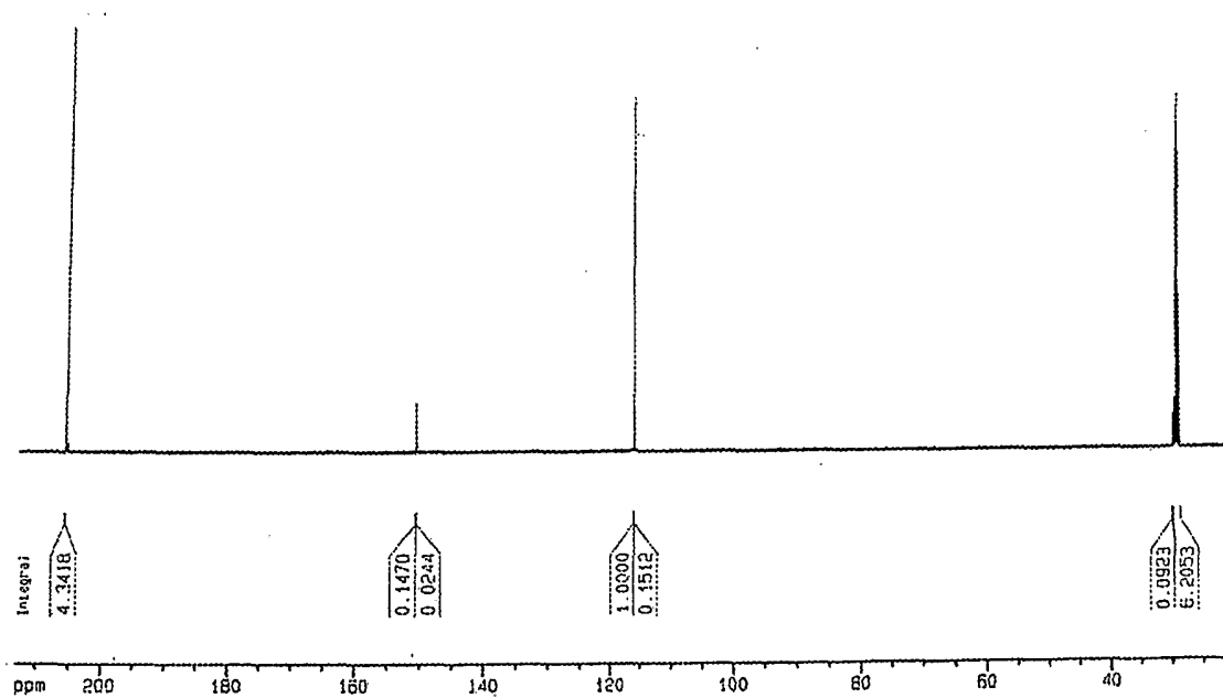
Fig 28. C-NMR spectroscopic profile of hydroquinone in CD 3 COCD 3
