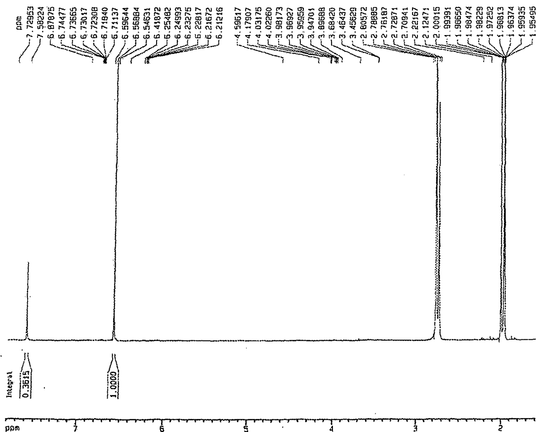
Fig 26. H-NMR spectroscopic profile of the cs-oxidant after reduction with sodium dithionite.
