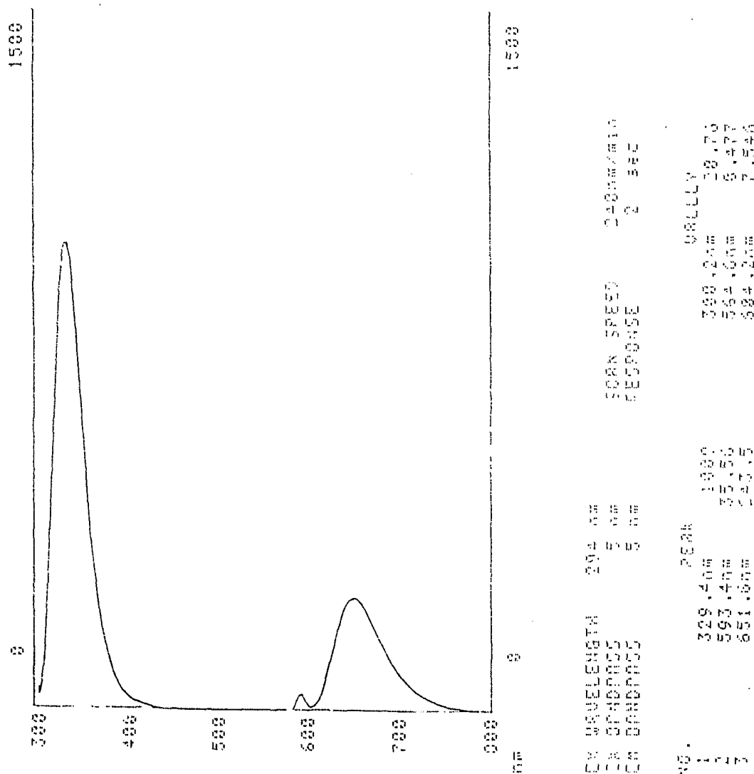
Fig 20. Fluorescence spectroscopic profile of the hydroquinone in methanol. The excitation was at 294 nm and the emission scanning was measured from 300 nm to 800 nm. The emission maxima were at 329.4 nm and at 651.6 nm.
