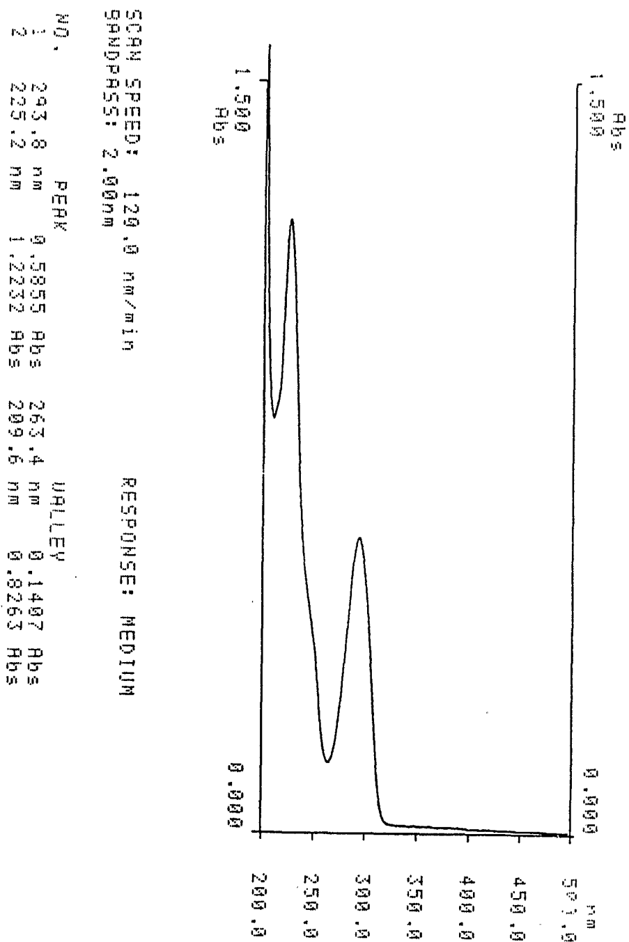
Fig 19. UV spectrophotometric profile of equimolar mixture of p-benzoquinone and hydroquinone in methanol. There is a shoulder near 242 nm ( the \lambda_{max} of p-benzoquinone).
