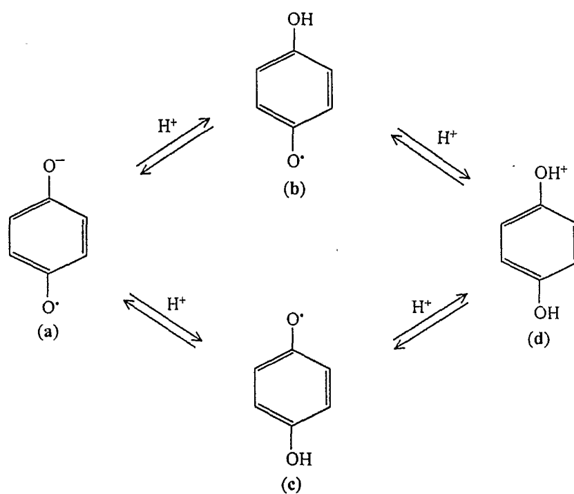
Fig 1. Mesomeric forms of p-benzo-semiquinone. (a) anionic; (b),(c) neutral; (d) cationic.
