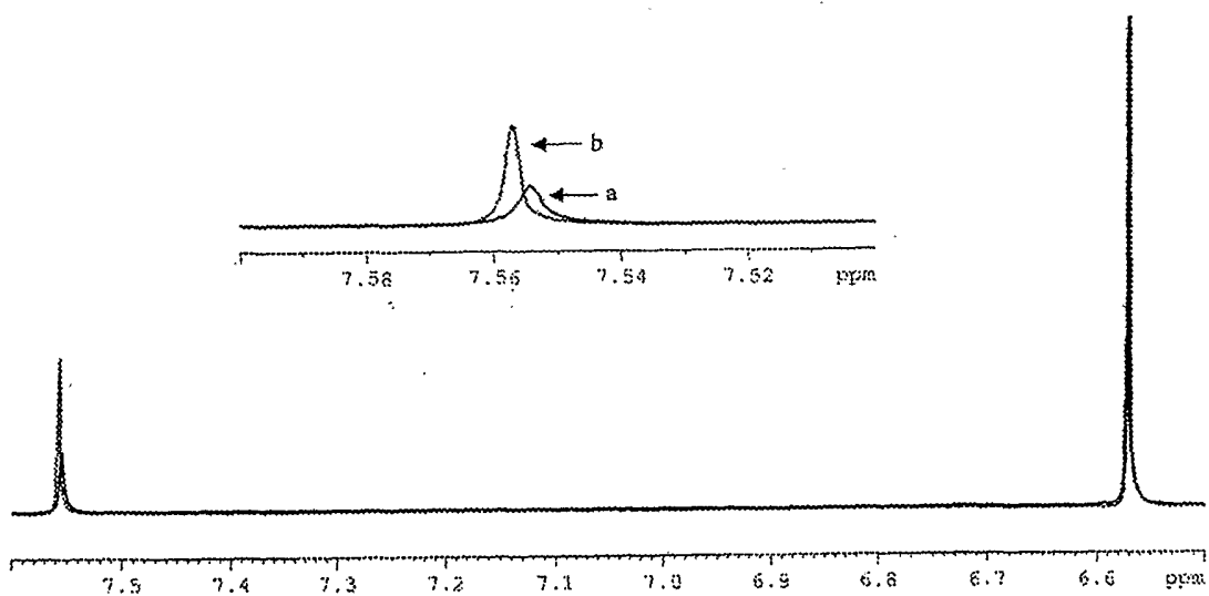
Fig 25. Comparative H-NMR spectroscopic profiles of (a) cs-oxidant and (b) hydroquinone.
