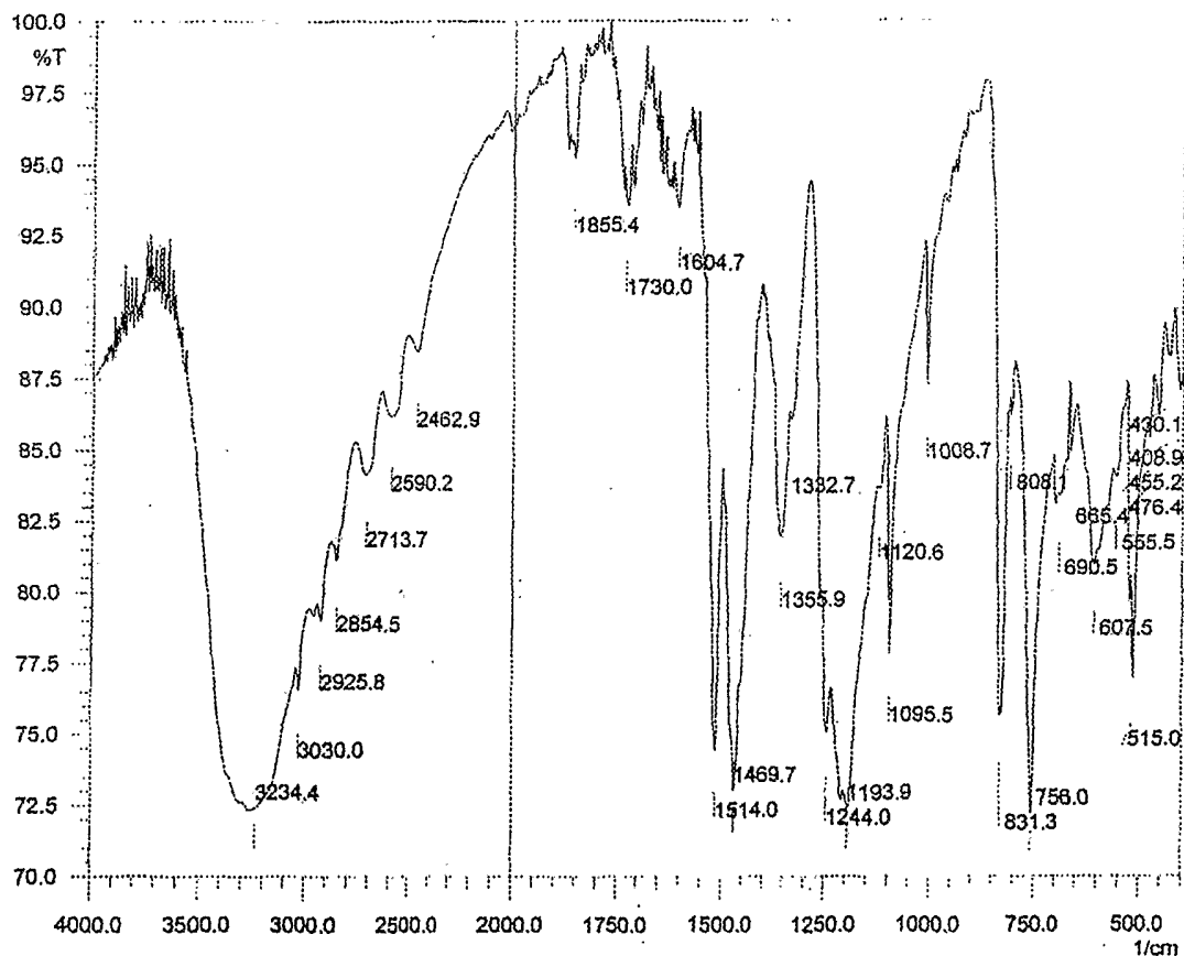
Fig 21. FTIR spectroscopic profile of the cs-oxidant.
