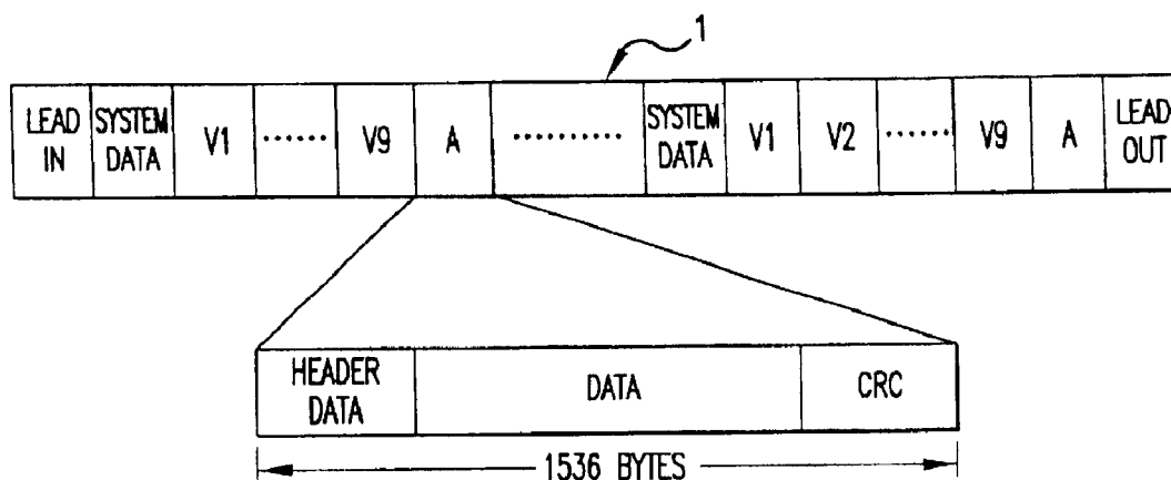
FIG. 2 CONVENTIONAL ART
