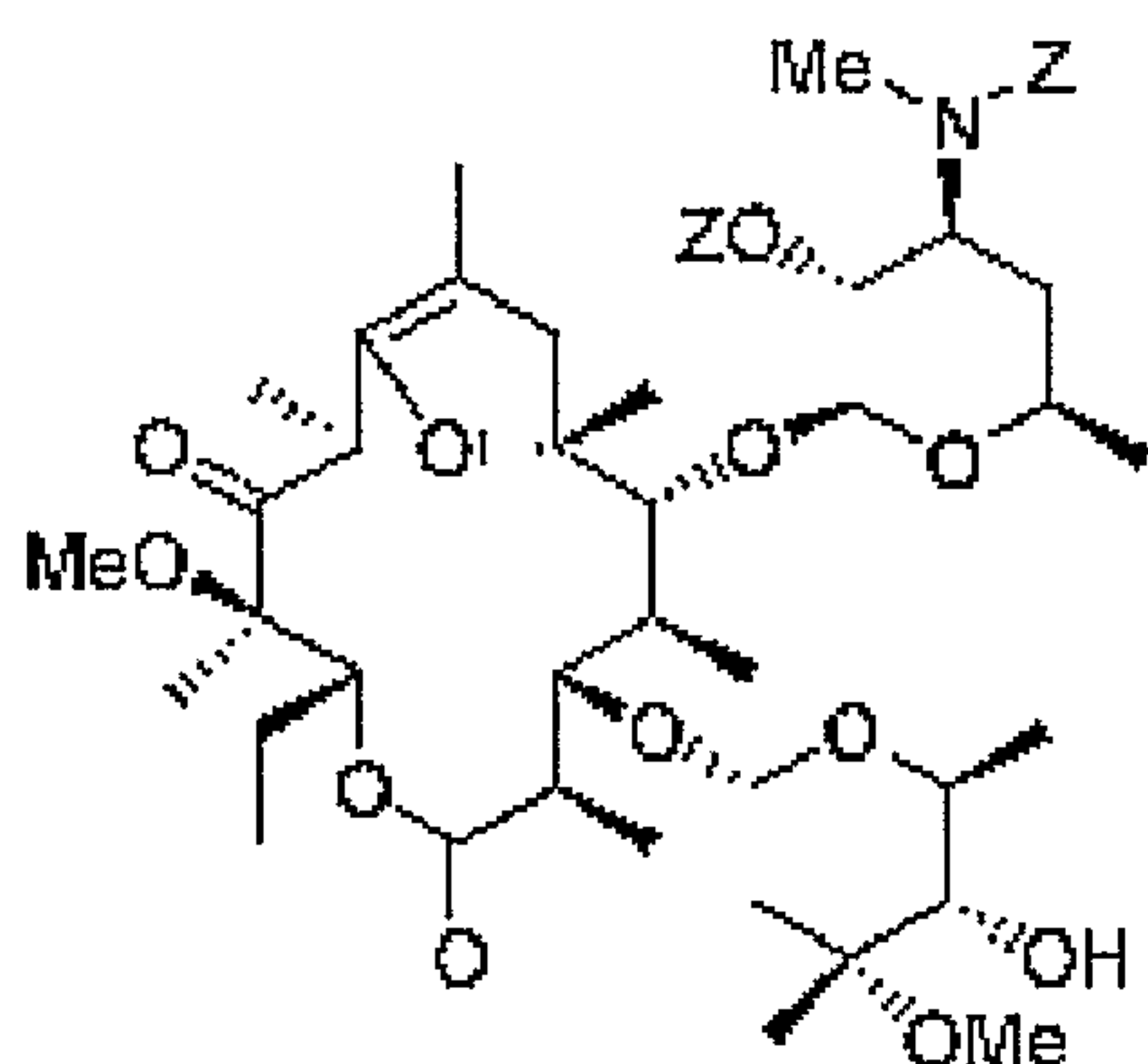
Compound 2
