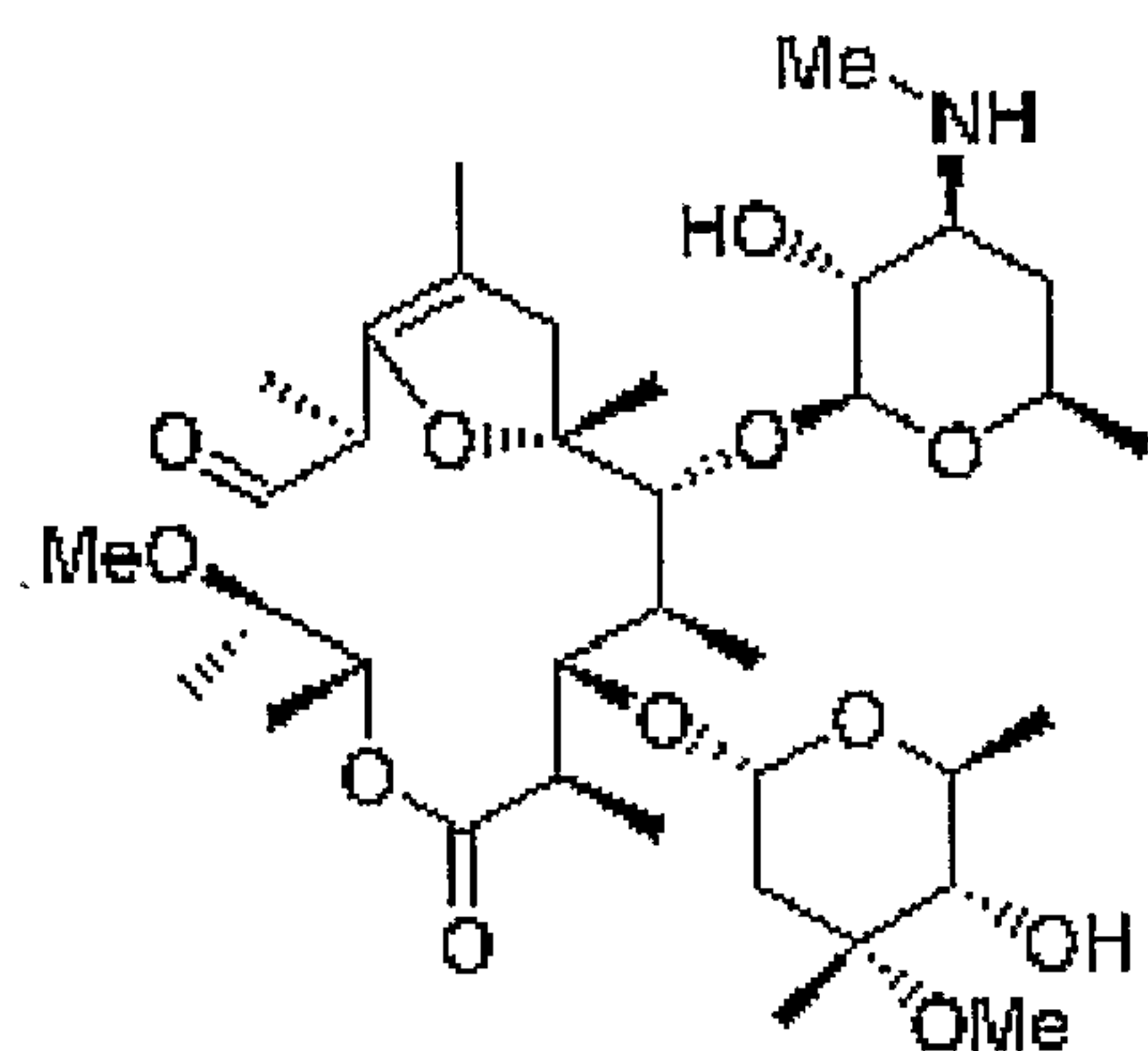
Compound 3
