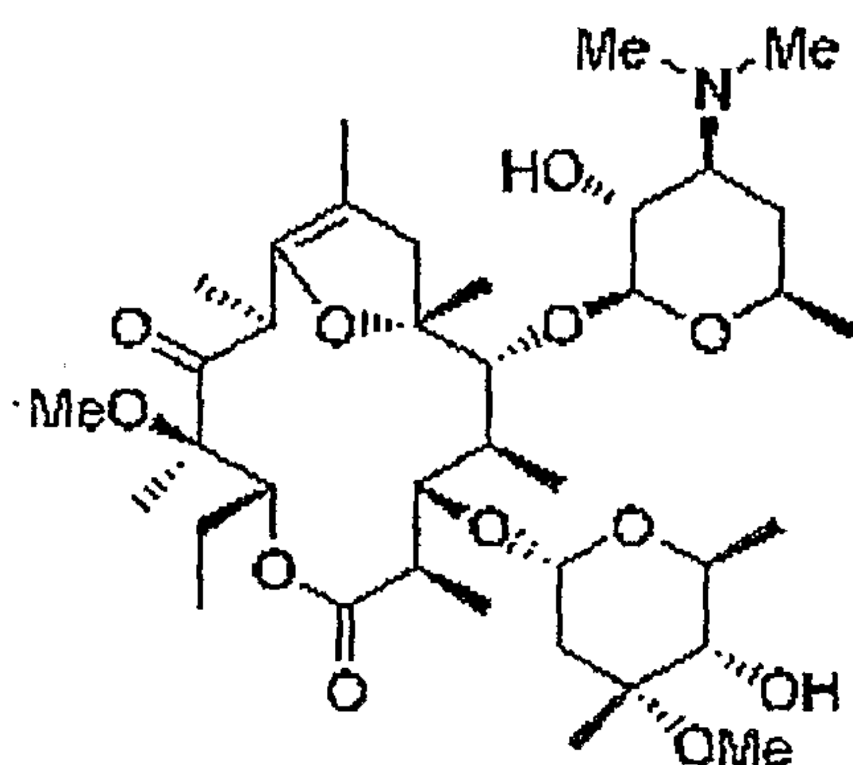
Compound 1
