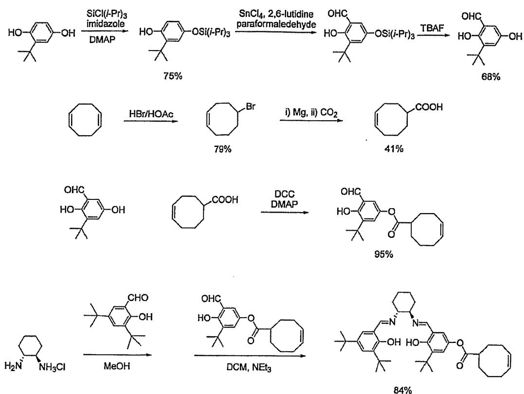
Scheme 4. Synthesis of cyclooctene-functionalized salen ligands.
