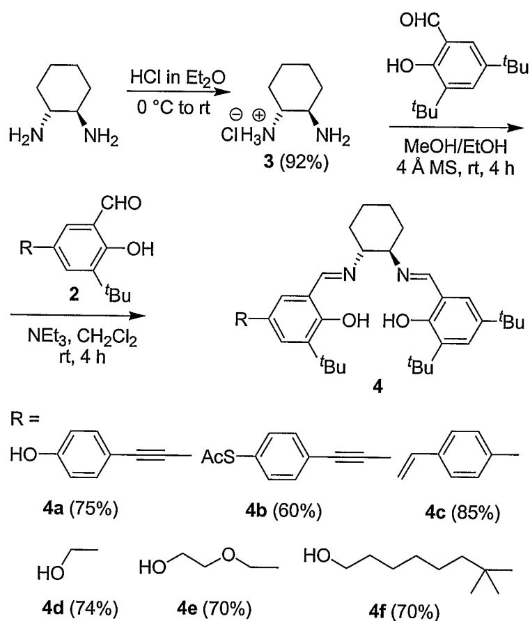
Scheme 2. Synthesis of unsymmetrical salen ligands.
