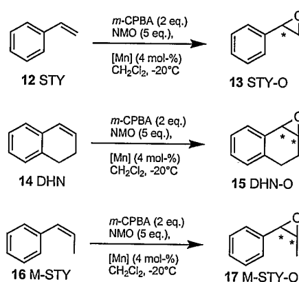
Scheme 11. Epoxidations of unfunctionalized olefins.
