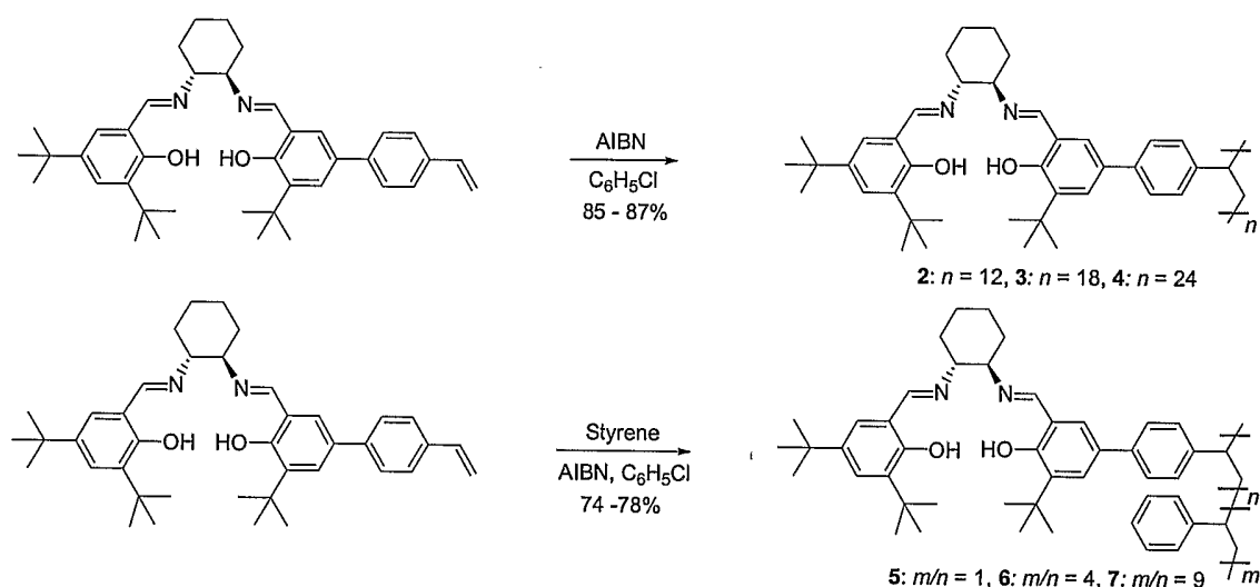
Scheme 7. Synthesis of homopolymeric salen ligands and co-polymeric polystyrene-supported salen ligands.
