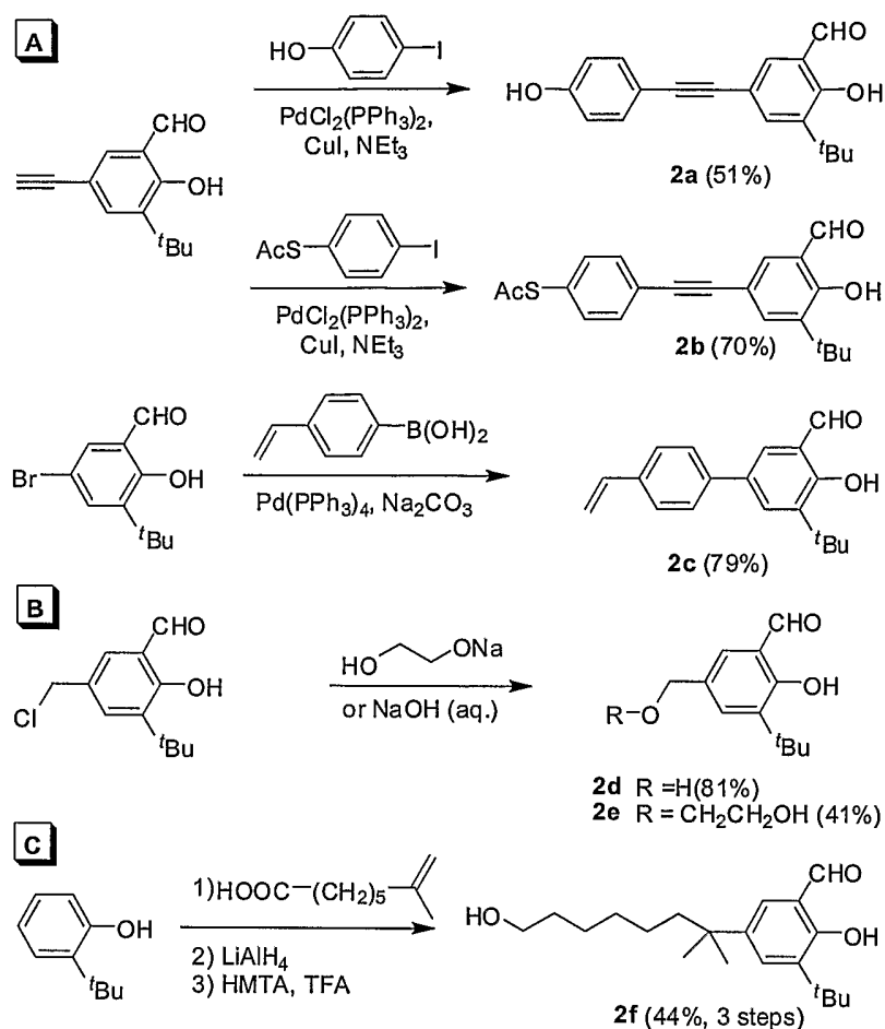
Scheme 1. Synthesis of the salicylaldehydes 2.
