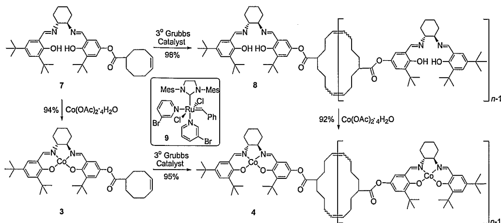
Scheme 9. Synthesis of oligomeric salens and oligomeric Co(salen) complexes via ring-expanded olefin metathesis of cyclooctene substituted salen monomers.
