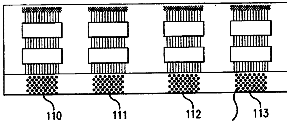
FIG. 11A AREA ARRAY CONTACT PADS
