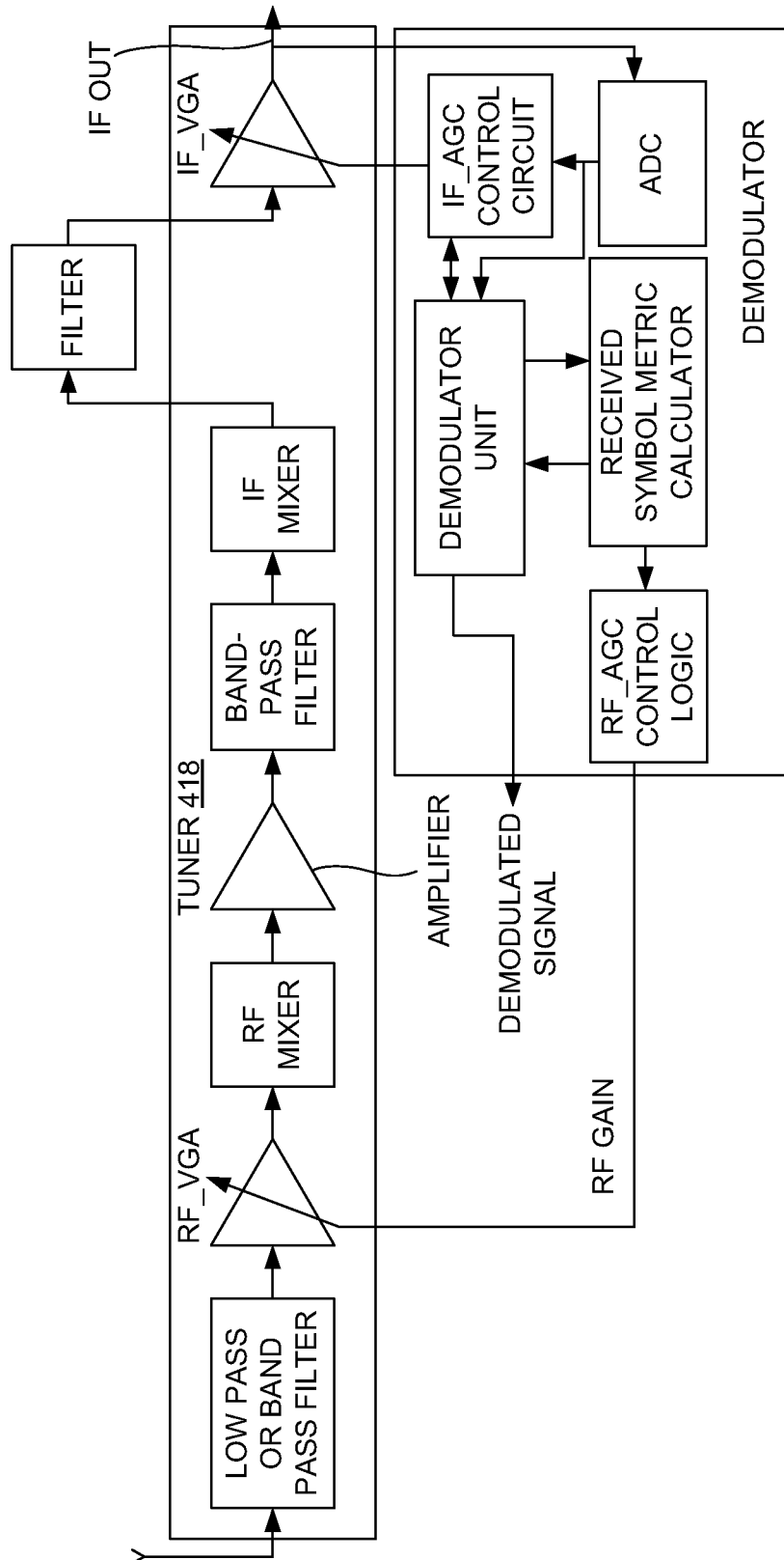
FIG. 4C (PRIOR ART)
