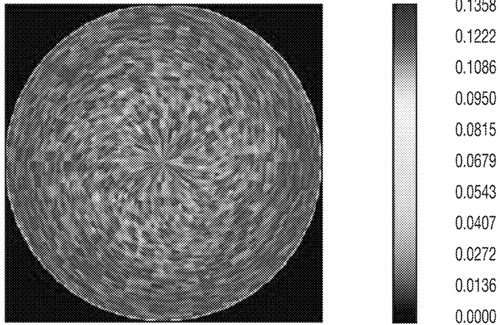
Irradiance with Baffle
