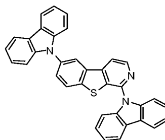
Compound D:
