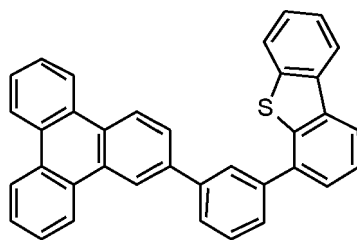
Compound G:
