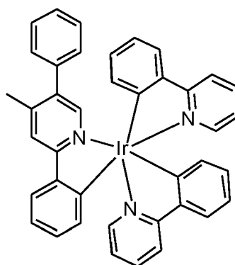
Compound G:
