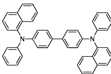
Compound B:
