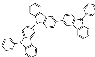
Compound C:
