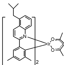
Compound E:
