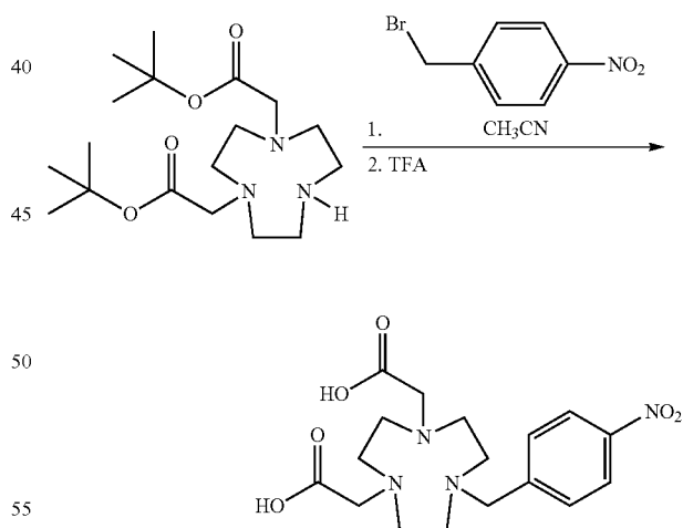
Scheme 3: Synthesis of NODA-MPN
