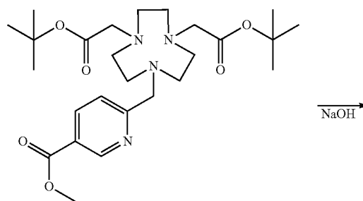
Scheme 23. Hydrolysis of the methyl ester
