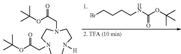
Scheme 15: Synthesis of NODA-BAMA
