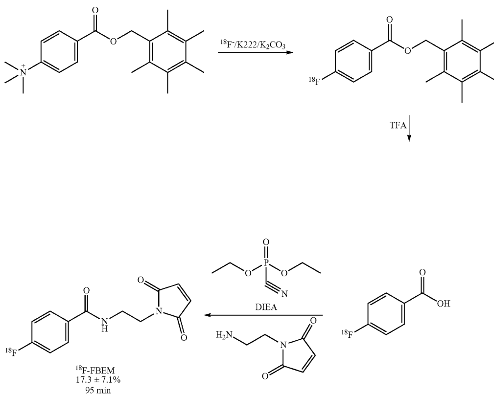
Scheme 20: Synthesis of ^{18}\text{F} -FBEM
