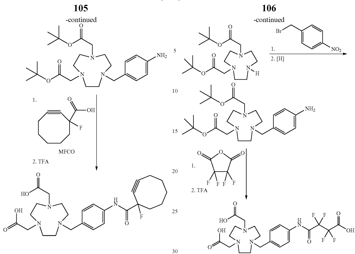
Scheme 18: Synthesis of NODA-MPAFSA
