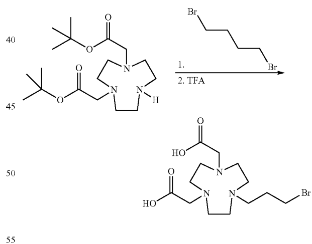
Scheme 9: Synthesis of NODA-MBEM
