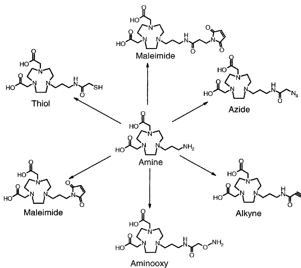
NODA-propyl amine derived BFCs
