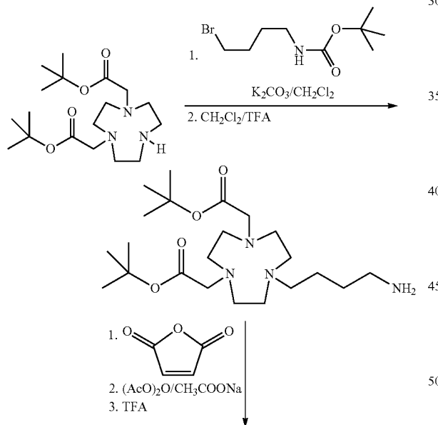
Scheme 10: Synthesis of NODA-BM
