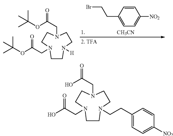
Scheme 4: Synthesis of NODA-EPN
