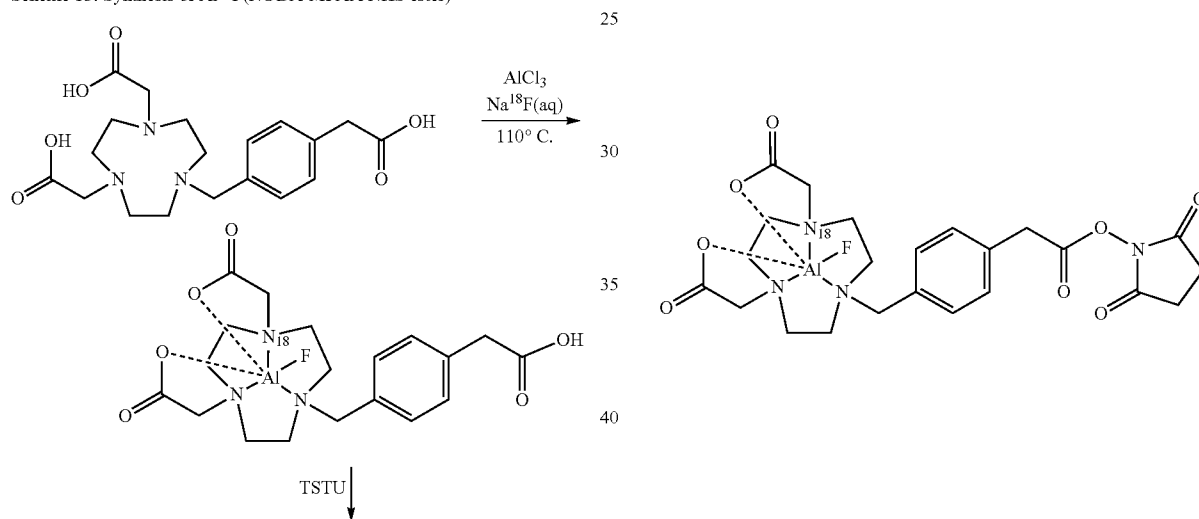
Scheme 13: Synthesis of \text{Al}^{18}\text{F}(\text{NODA-MPAA NHS ester})
