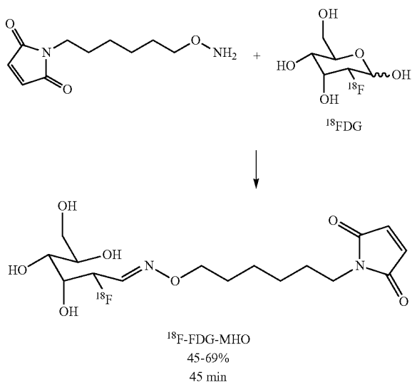
Scheme 21: Synthesis of ^{18}\text{F} -FDG-MHO
