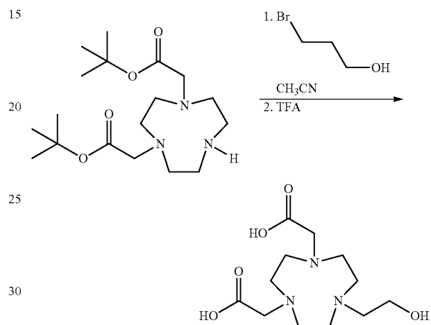
Scheme 7: Synthesis of NODA-Ethanol
