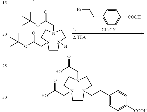
Scheme 2: Synthesis of NODA-EBA
