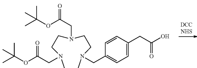
Scheme 19: Synthesis of Al 18 F(NODA-MPAEM)
