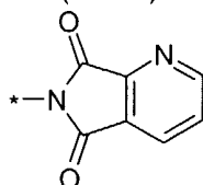
pyrrolo[3,4-b]pyridin- 5,7-dion-6-yl
