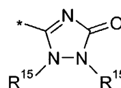
1,2,4-triazol-3-on-5-yl (7.0.3)
