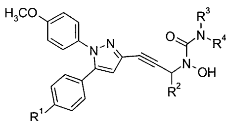
(5.2.4)
