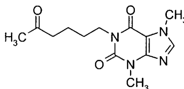
Pentoxifylline
