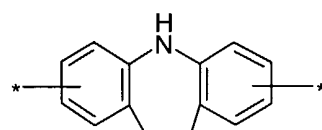
(1.2.29)
