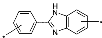
(1.2.28)
