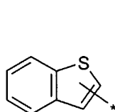
Benzothieryl
