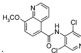
D4418
