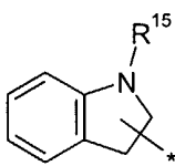
indolinyl
