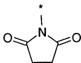
Succinimid-1-yl
