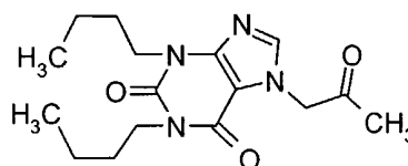
Denbufylline
