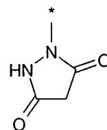
pyrazolidin-3,5-dion-1-yl (1.7.23)
