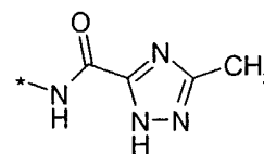
(8.0.4)
