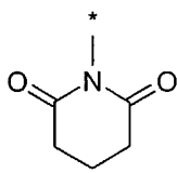
glutarimid-1-yl
