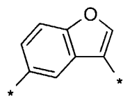
(3.0.73)
