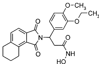
CDC-801
