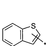
benzothieryl
