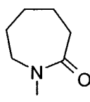
2H-azepin-2-on-1-yl
