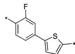
(3.0.18)
