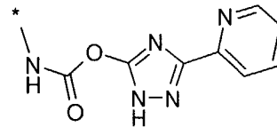
(8.0.7)
