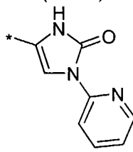
(4.8.26)
