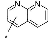
1,8-naphthyridinyl
