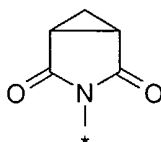
3-azabicyclo[3.1.0]-hexane-2,4-dion-3-yl (1.7.21)
