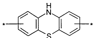
(1.2.28)
