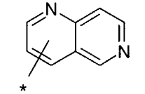
1,6-naphthyridinyl
