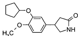
Rolipram (0.0.12)
