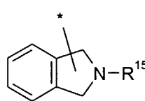
isoindolinyl (7.5.3)
