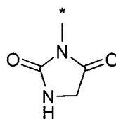
imidazolidin-2,4-dion-1-yl (1.7.11)
