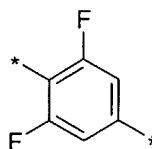
(2.5.3)
