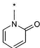
pyrid-2-on-1-yl (1.7.5)
