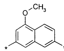
(3.0.6)
