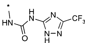
(8.0.5)
