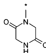
piperazin-2,5-dion-1-yl (1.7.12)
