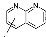
1,8-naphthyridiny
