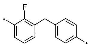
(3.0.13)
