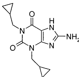
Cipamfylline
