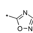
1,2,4-oxadiazol-5-yl
