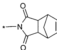
norborn-5-en-2,3-dicarboximid-1-yl
