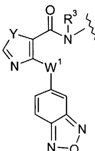
(1.0.16)
