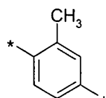
(2.5.34)
