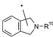
isoindolinyl
