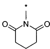
glutarimid-1-yl (1.7.2)
