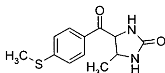
Enoximone (0.0.10)
