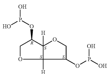
1,4:3,6-dianhydrobis(dihydrogenphosphite)hexitol
