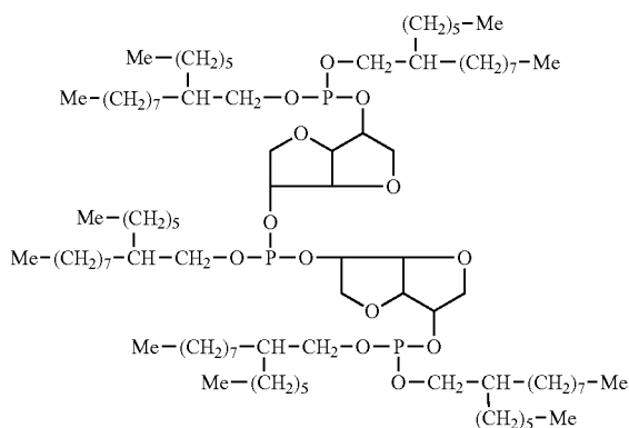
1,4:3,6-dianhydrohexitol 2,2'-(2-hexyldecyl phosphite)-5,5'-bis[bis(2-hexyldecyl) phosphite]
