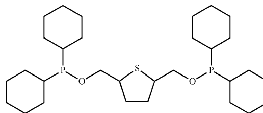
hexitol-2,3,4,5-tetra-deoxy-2,5-epithio bis(dicyclohexylphosphinite)
