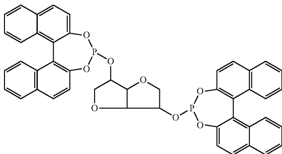
1,4:3,6-dianhydro-2,5-bis-O-[(11bR)dinaphtho[2,1-d:1',2'-f][1,3,2]dioxaphosphpin-4-yl]hexitol
