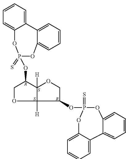
1,4:3,6-dianhydro-2,5-bis-O-(6-sulfidodibenzo[d,f][1,3,2]dioxaphosphpin-6-yl)hexitol
