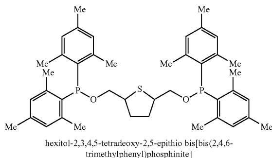
hexitol-2,3,4,5-tetra-deoxy-2,5-epithio bis(diphenylphosphinite)
