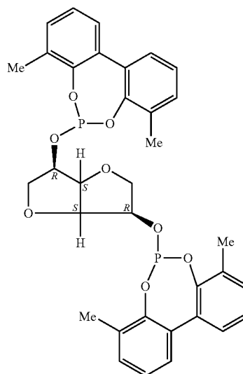
1,4:3,6-dianhydro-2,5-bis-O-(4,8-dimethyldibenzo[d,f][1,3,2]dioxaphosphpin-6-yl)hexitol
