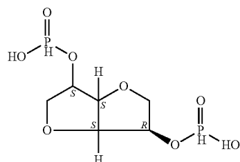
1,4:3,6-dianhydrohexitol bis(hydrogenphosphonate)
