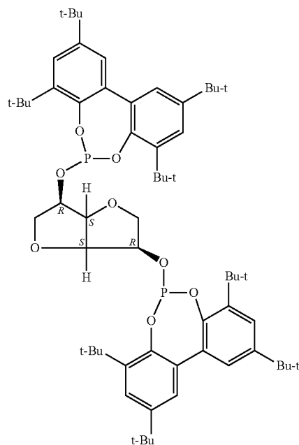
1,4:3,6-dianhydro-2,5-bis-O-[2,4,8,10-tetrakis(1,1-dimethylethyl)dibenzo[d,f][1,3,2]dioxaphosphpin-6-yl]hexitol
