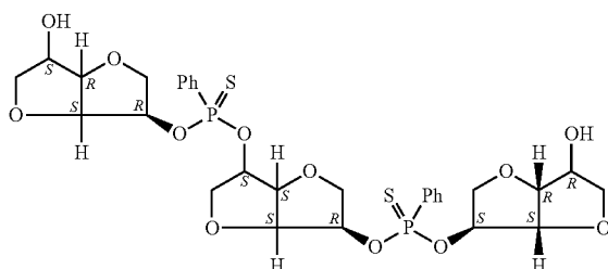
1,4:3,6-dianhydro-D-glucitol-2,5':2',5''-bis(phenylphosphonothioate)
