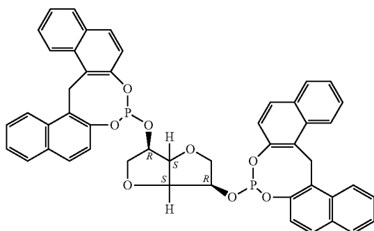
1,4:3,6-dianhydro-2,5-bis-O-(16H-dinaphtho[2,1-d:1',2'-g][1,3,2]dioxaphosphocin-8-yl)hexitol
