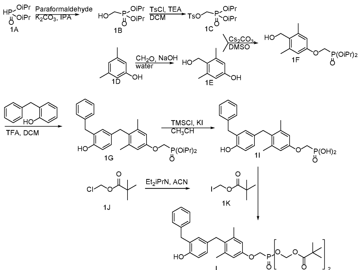
SCHEME 1
