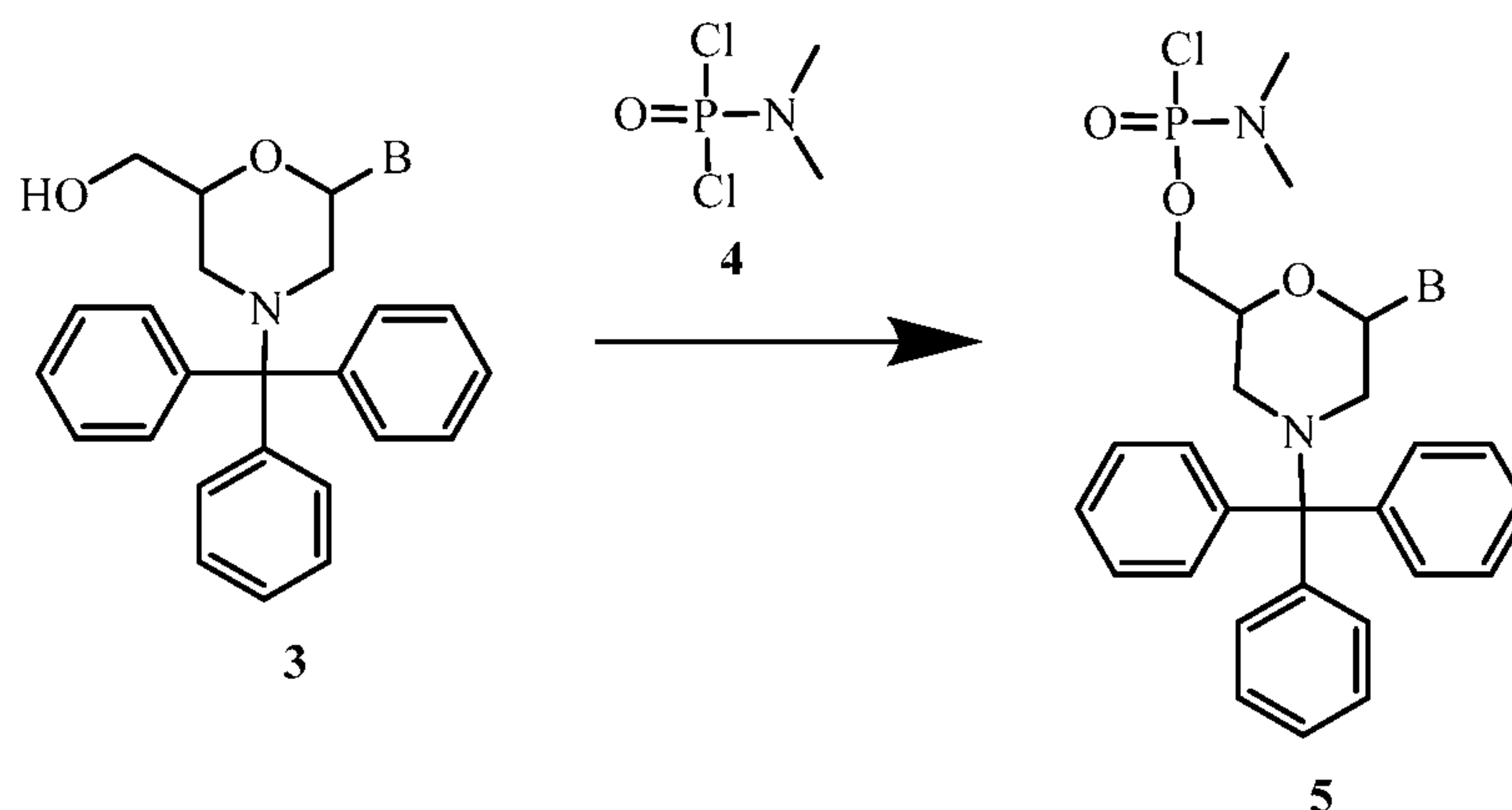
Scheme 1: General synthetic route to PMO Subunits
