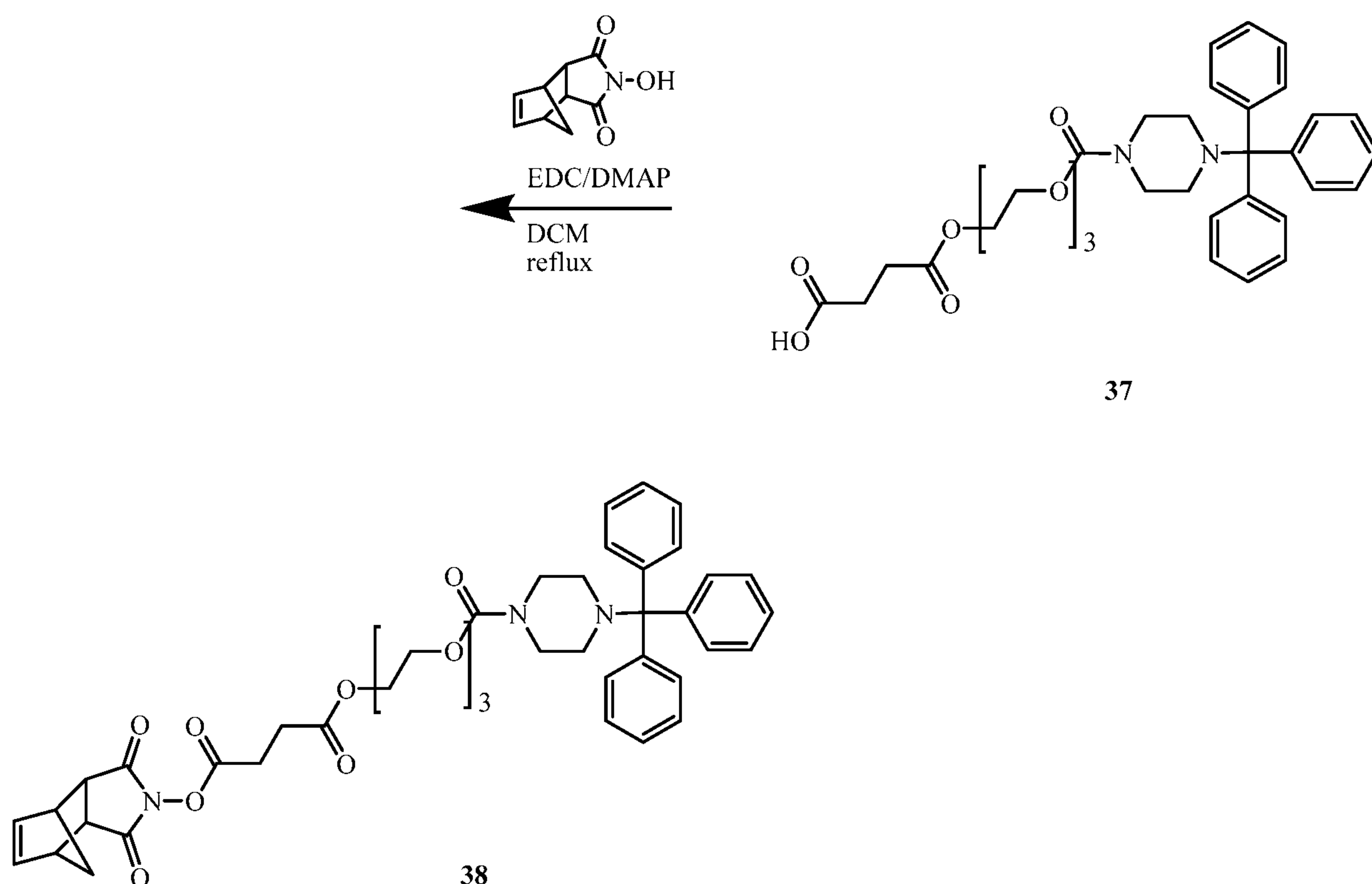
Scheme 2: Preparation of Activated Tail Acid
