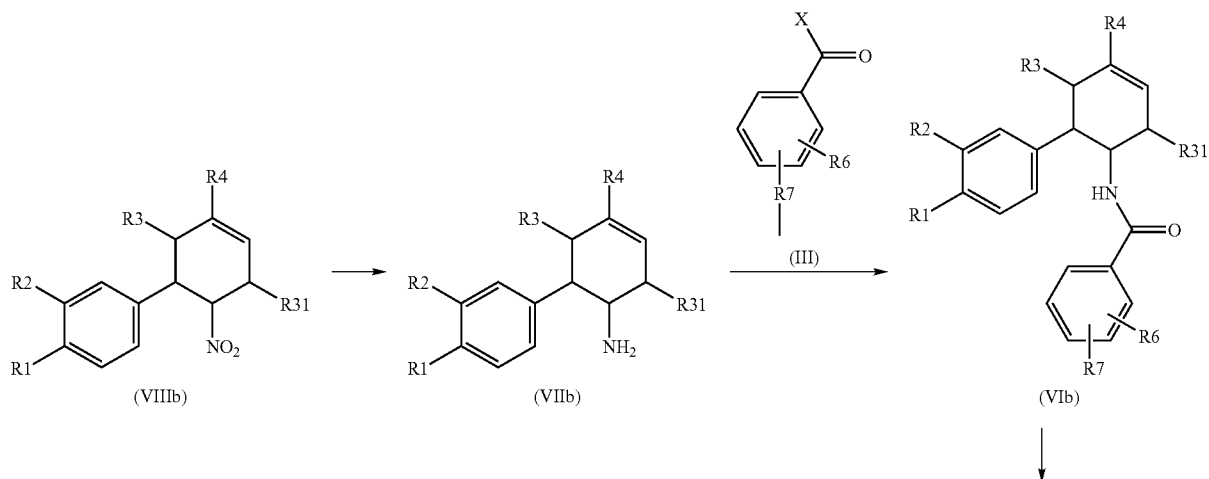
Reaction scheme 3:
