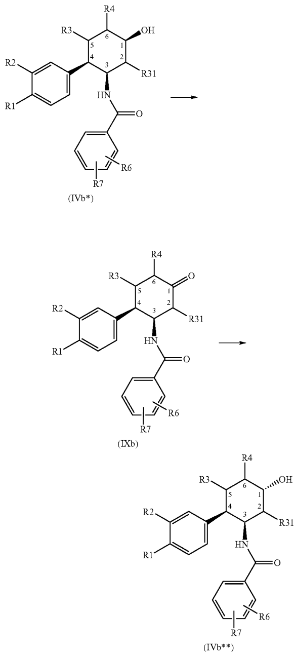
Reaction scheme 4:
