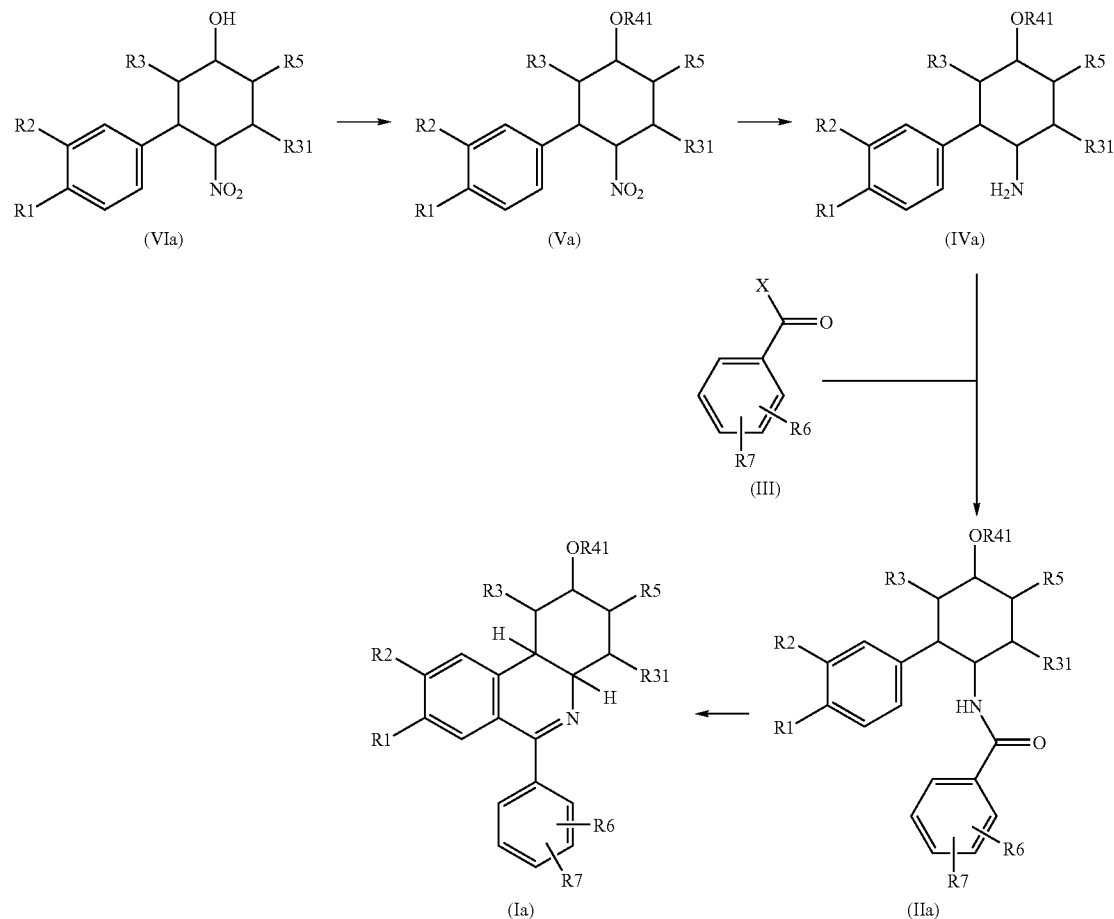
Reaction scheme 1:
