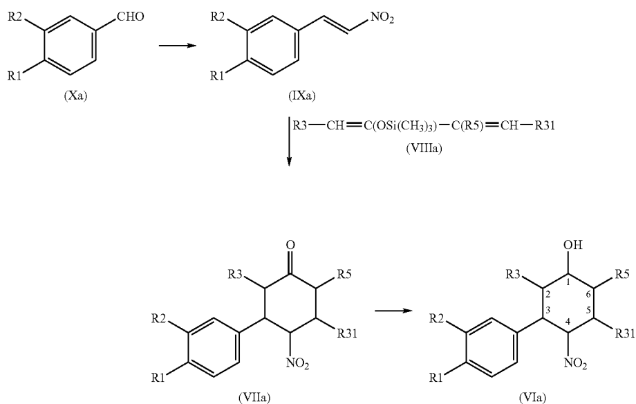
Reaction scheme 2:
