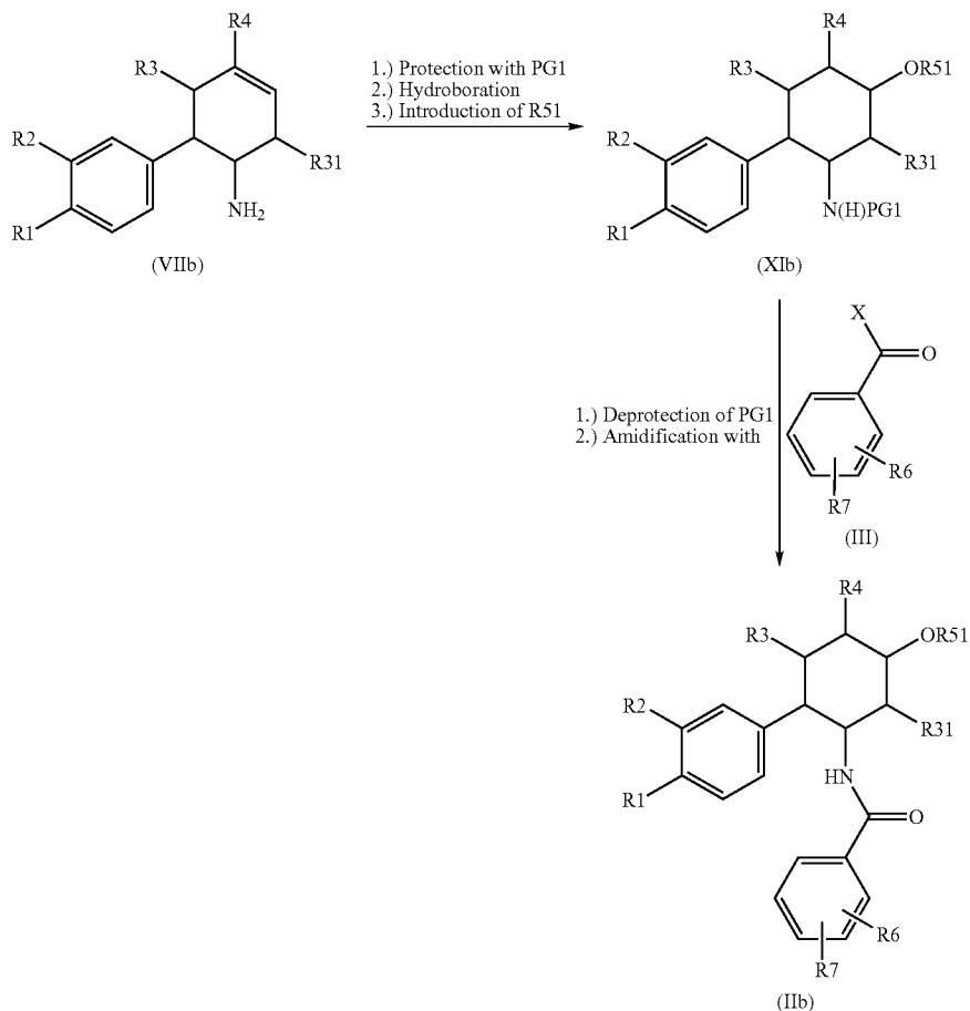
Reaction scheme 6:
