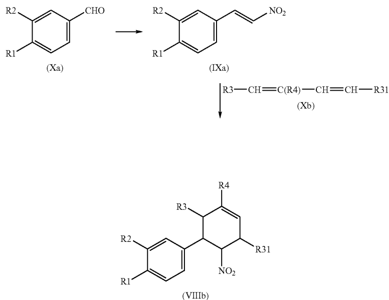
Reaction scheme 5:
