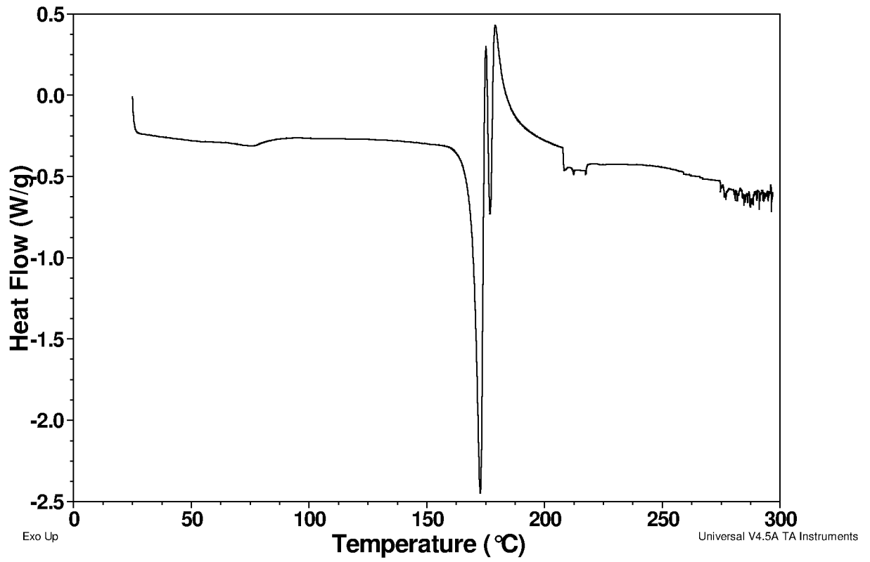
Figure L: DSC Thermogram of Compound A: 6-hydroxy-2-naphthoic acid (1:1) co-crystal, Form B
