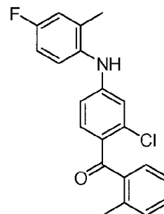
(2-chloro-4-(4-fluoro-2-methylphenylamino)phenyl)(o-tolyl)methanone
