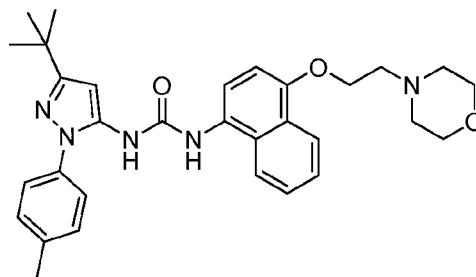
BIRB 796 (Doramapimod)
