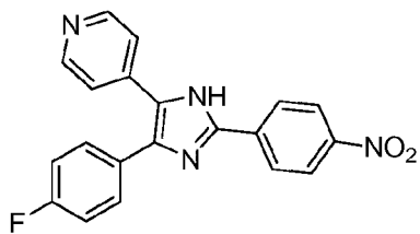
PD 169316
