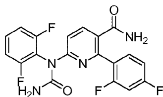
VX-702
