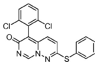
VX-745
