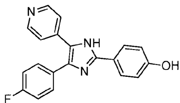
SB 202190
