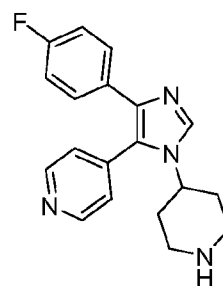
4-(4-(4-fluorophenyl)-1-(piperidin-4-yl)-1H-imidazol-5-yl)pyridine
