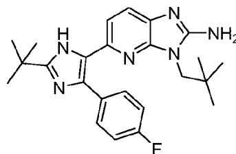
LY2228820
