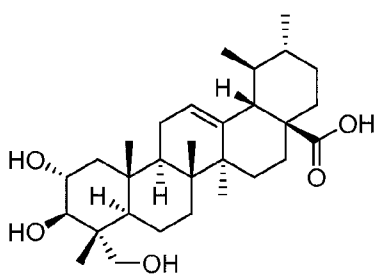
Asiatic acid
