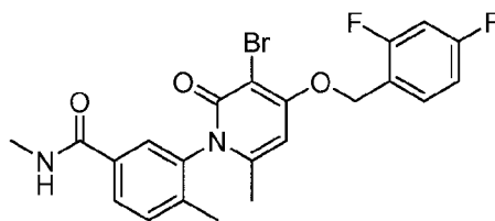
PH-797804
