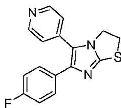
SKF 86002
