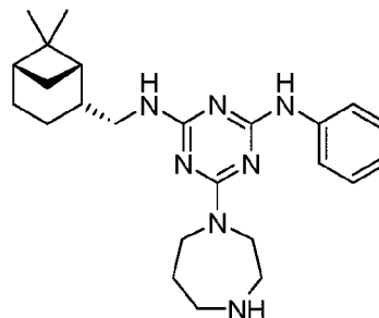
6-(1,4-diazepan-1-yl)-N²-(((1S,2R,5S)-6,6-dimethylbicyclo[3.1.1]heptan-2-yl)methyl)-N4-phenyl-1,3,5-triazine-2,4-diamine
