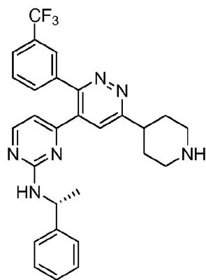
(R)-N-(1-phenylethyl)-4-(6-(piperidin-4-yl)-3-(3-(trifluoromethyl)phenyl)pyridazin-4-yl)pyrimidin-2-amine
