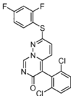
5-(2,6-dichlorophenyl)-2-(2,4-difluorophenylthio)-6H-pyrimido[1,6-b]pyridazin-6-one
