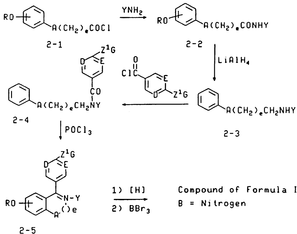
SCHEME 2
