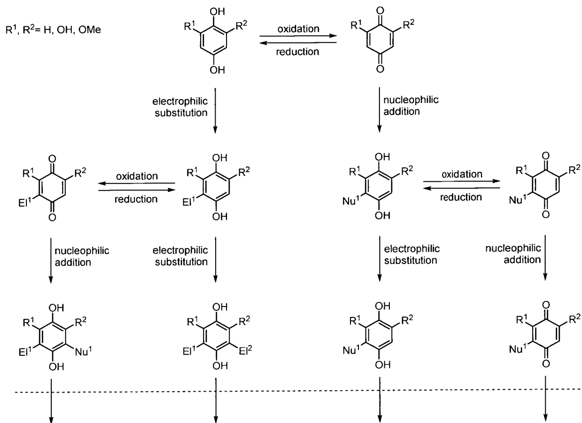
Scheme 1:
