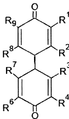
(VI d)
