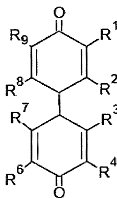
(VI d)
