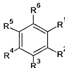
(X),
