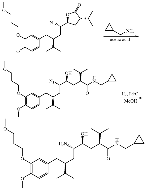
(2S,4S,5S,7S)-5-Amino-4-hydroxy-2-isopropyl-7-[4-methoxy-3-(3-methoxy-propoxy)-benzyl]-8-methyl-nonanoic acid cyclopropylmethyl-amide
