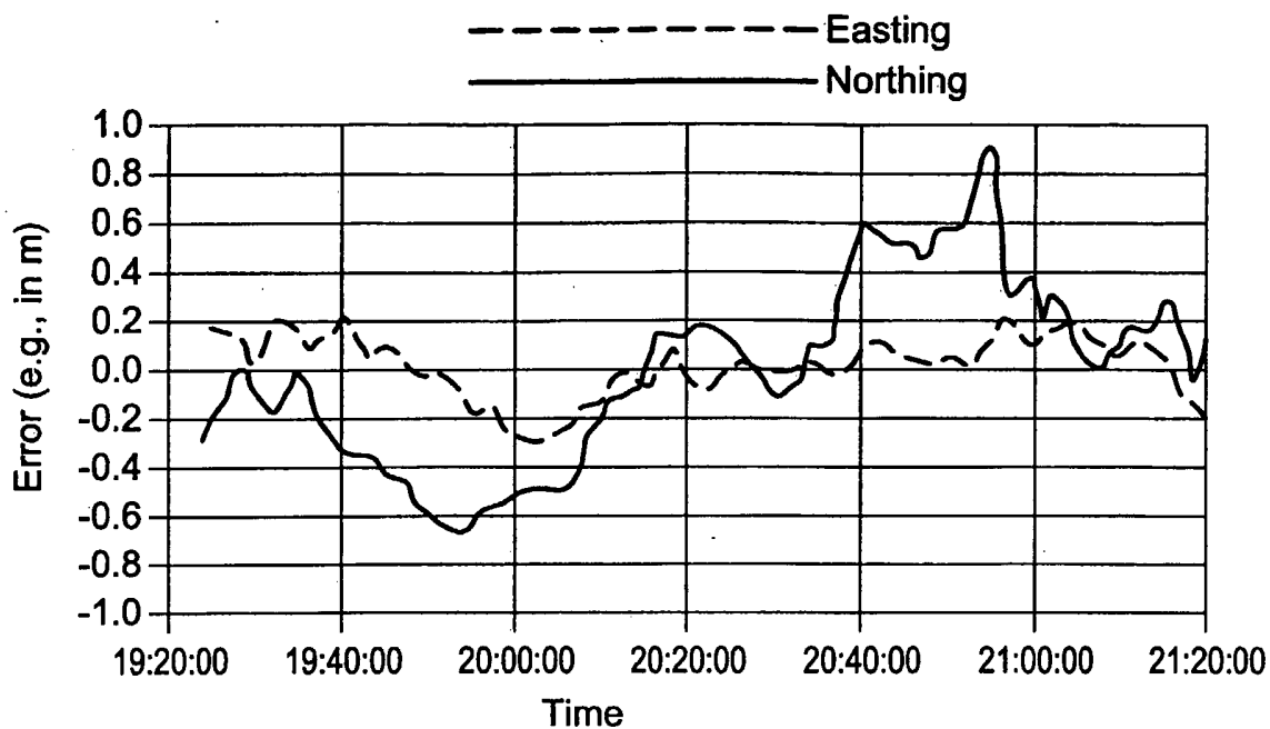
Fig. 12 DGPS Static Positioning Error
