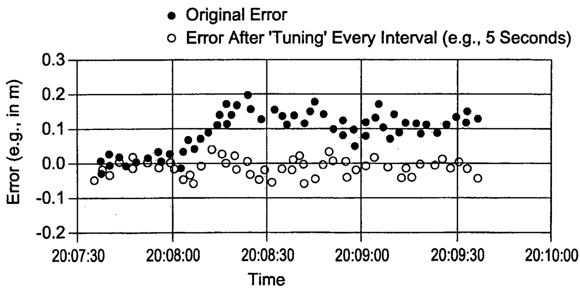
Fig. 13 DGPS by "Tuning" Positioning Error
