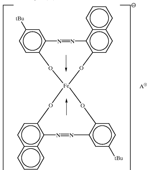
Azo iron complex (13):
