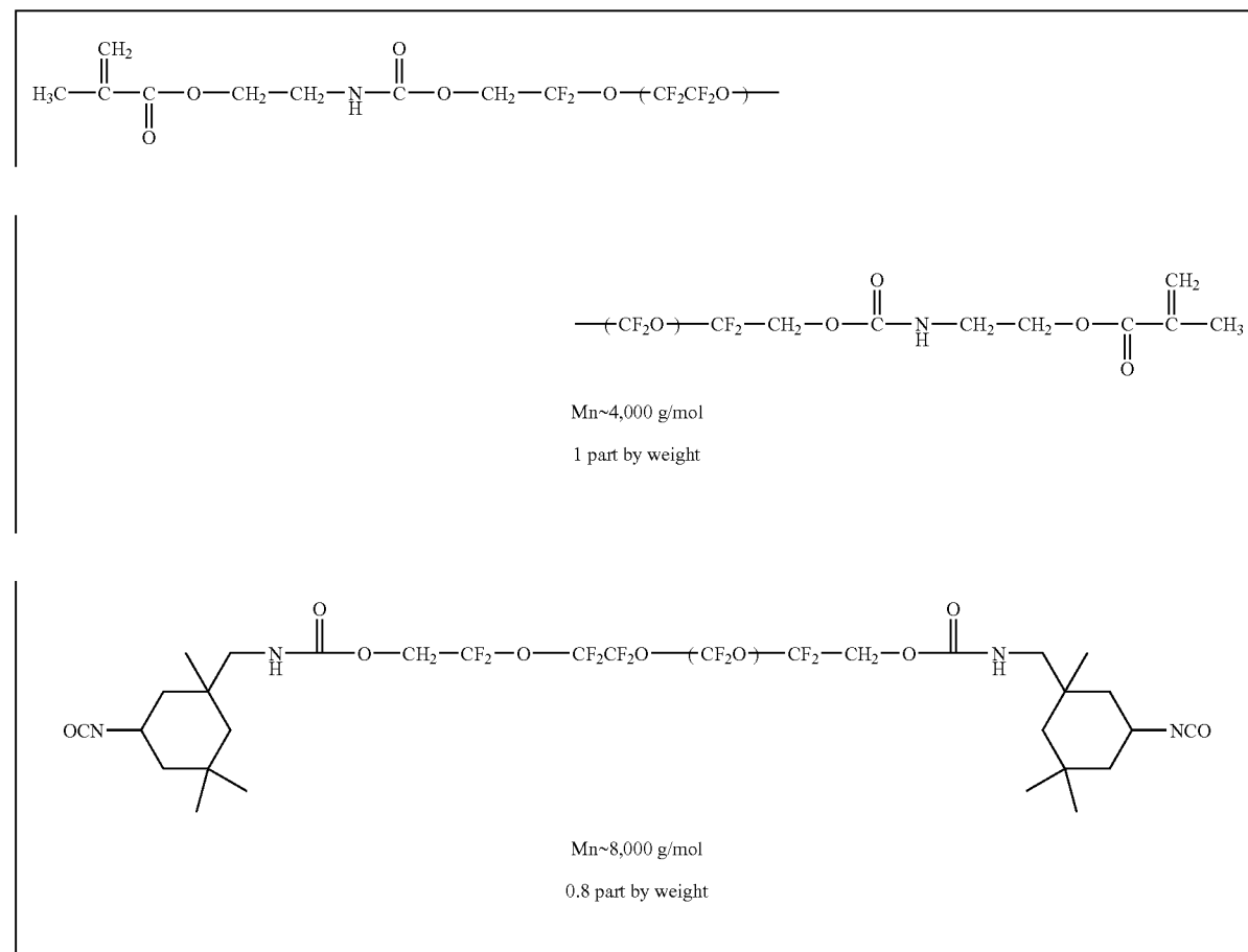
Scheme 1 - PFPE Dual Cure Composition
