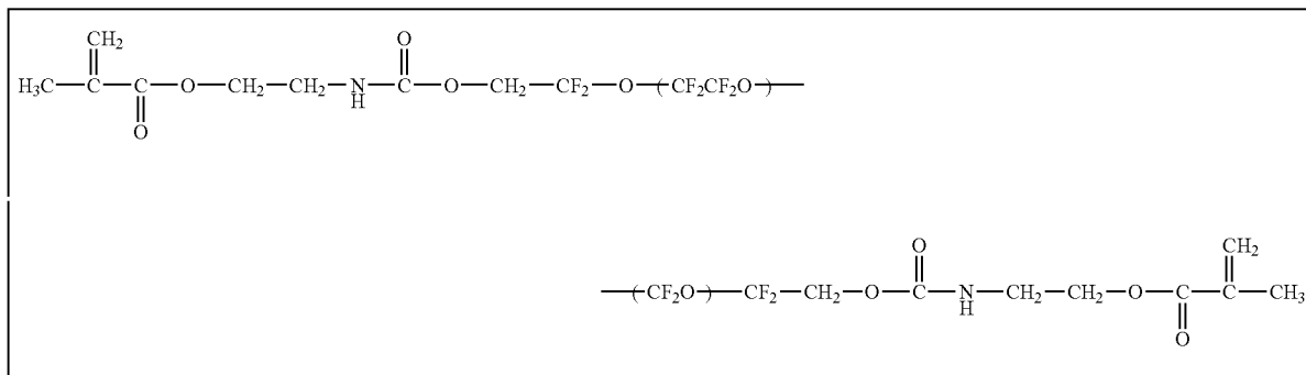
Scheme 2 of Example 1 - UV curable PFPE composition
