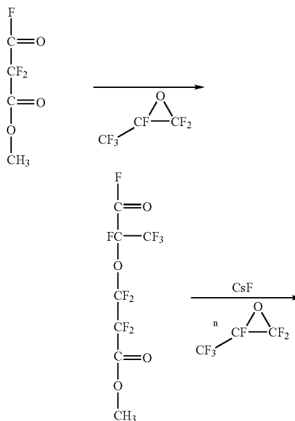
Scheme 3. Synthesis of a liquid PFPE precursor material from hexafluoropropylene oxide or tetrafluoro ethylene oxide.
