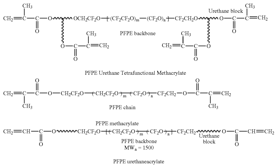
Scheme 6. PFPE Urethane Tetrafunctional Methacrylate
