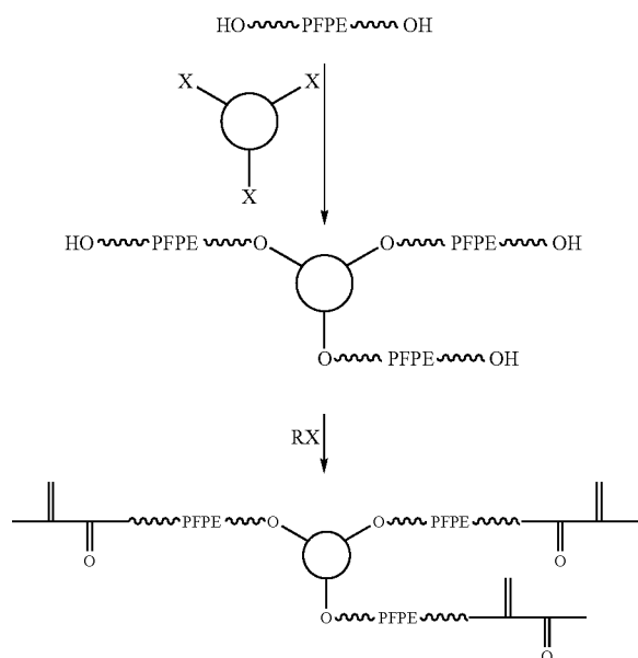
Scheme 4. Linker group joining three PFPE chains.
