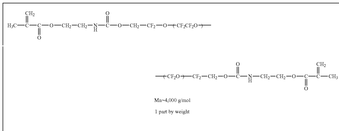
Scheme 1 of Example 1: PFPE Dual Cure Composition
