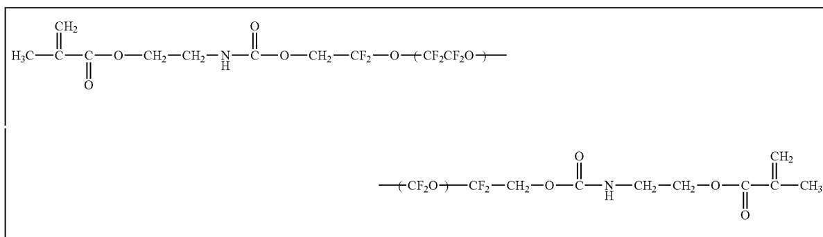
Scheme 2 - UV curable PFPE composition
