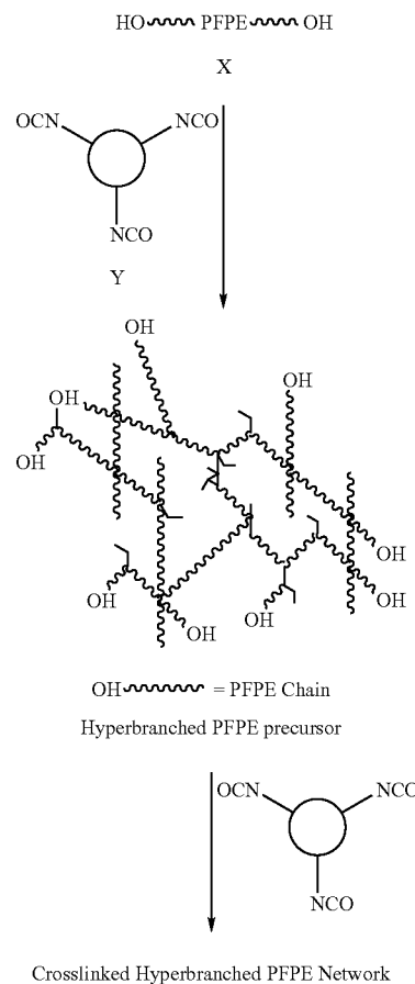
Scheme 5. Hyperbranched PFPE liquid precursor material.
