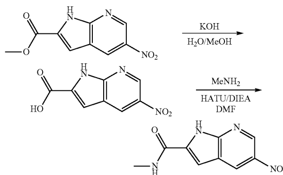
Scheme 17—General synthesis scheme of example AA
