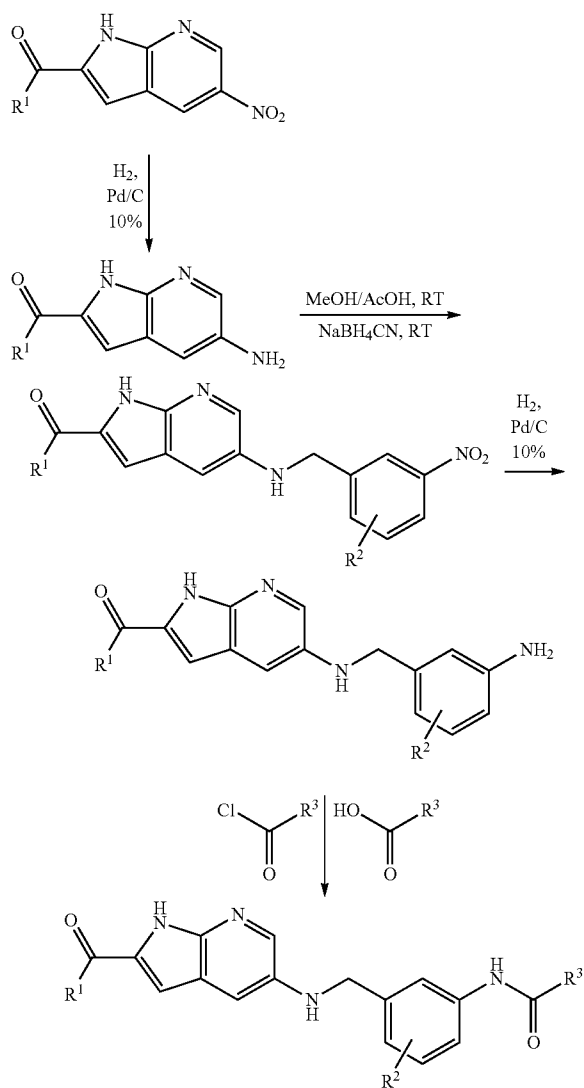
Scheme 18 - General synthesis scheme of example A
