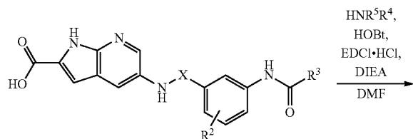
Scheme 29 - General synthesis scheme of example H
