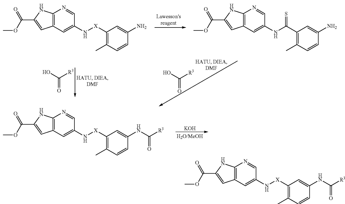
Scheme 28 - General synthesis scheme of example G
