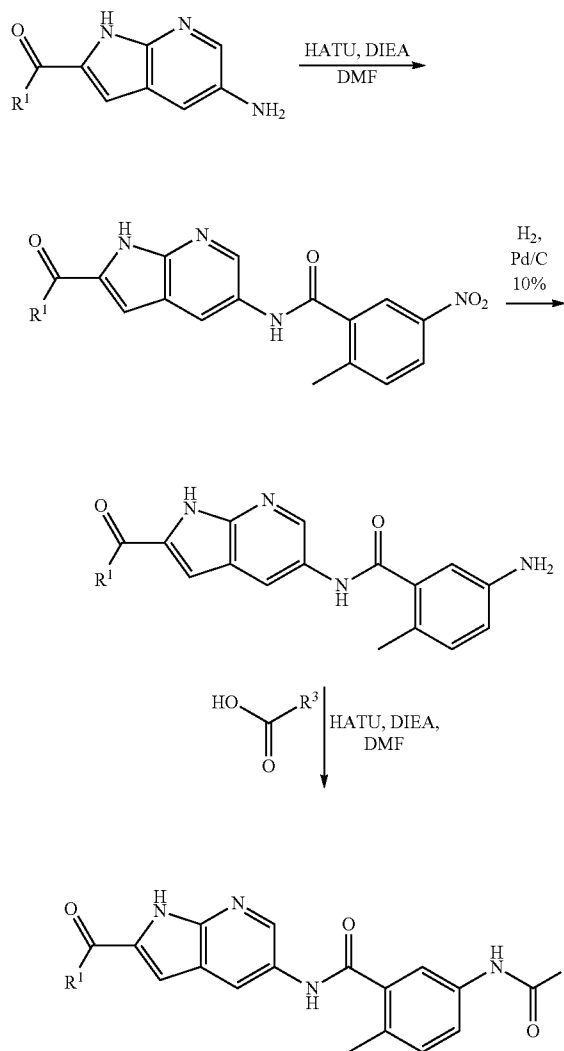
Scheme 23 - General synthesis scheme of example B
