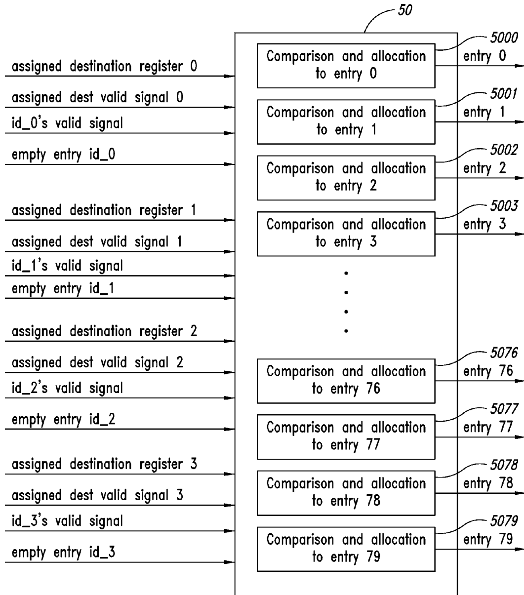
FIG. 2 (Prior Art)
