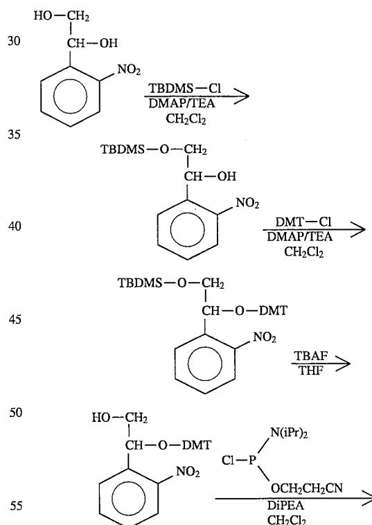
Scheme 2
