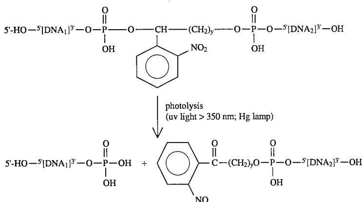
Scheme 4
