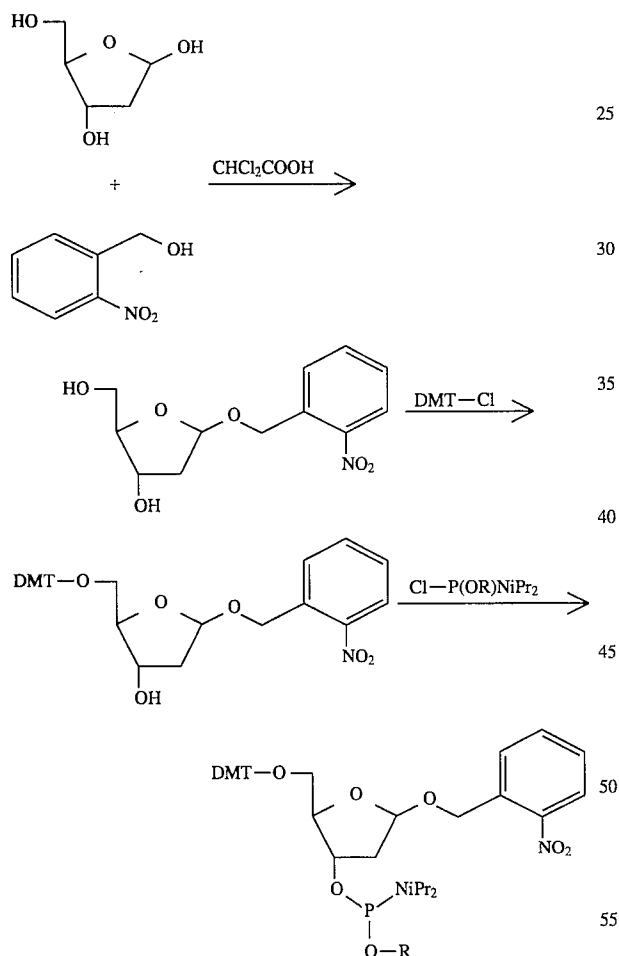
Scheme 5
