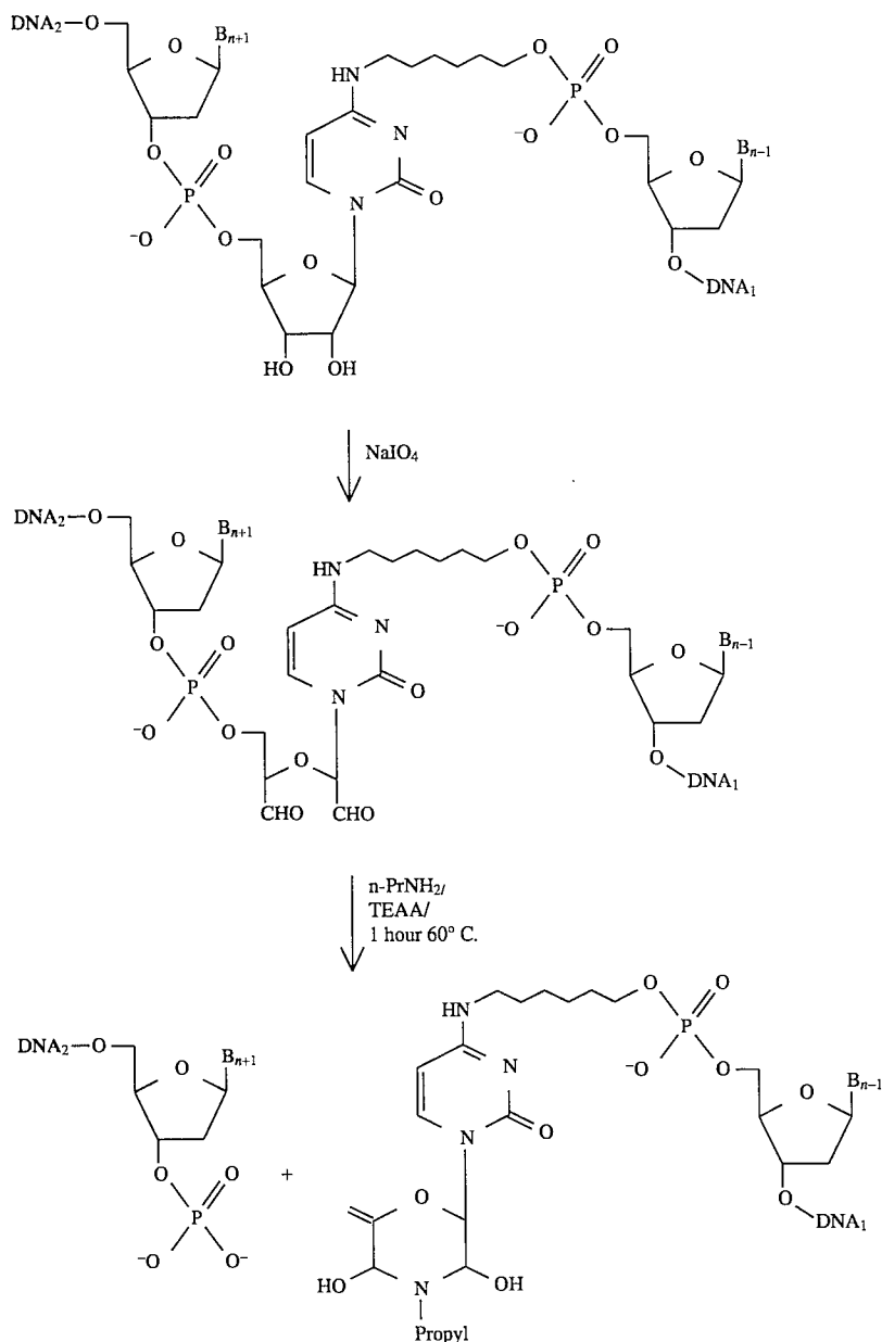
Scheme 7
