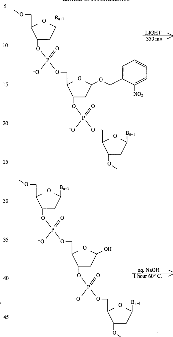
Scheme 6
