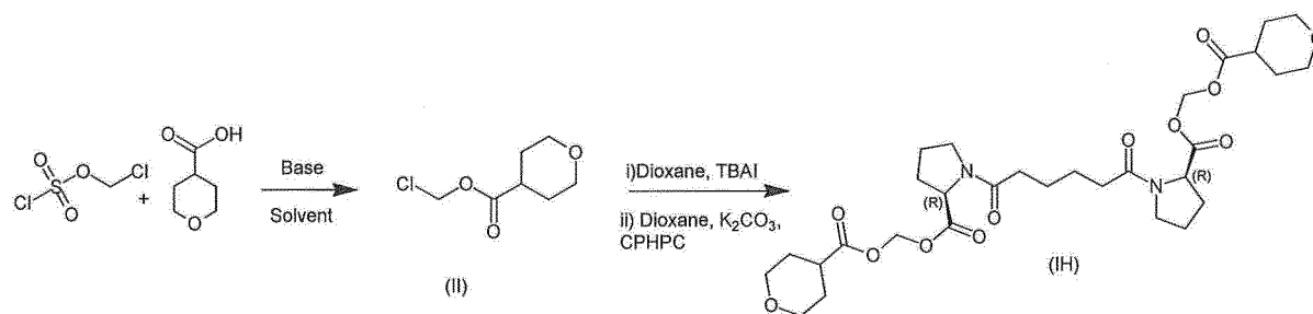
Reaction Scheme 1
