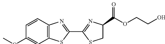
compound of formula XXXXV
