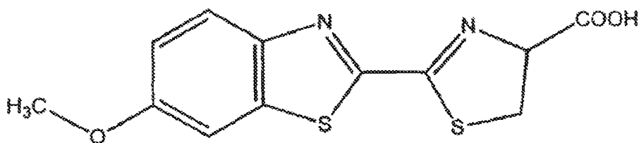
Luciferin 6' methyl ether (Luciferin-ME)
