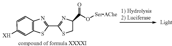
compound of formula XXXXI
