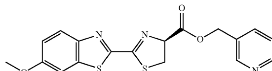
compound of formula XXXXVIII
