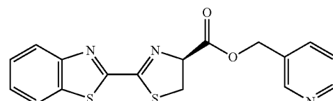
compound of formula XXXXIX
