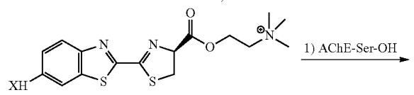
compound of formula XXXX
