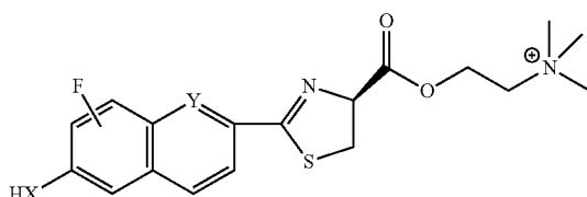
compound of formula XXXIX
