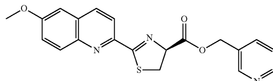
compound of formula L
