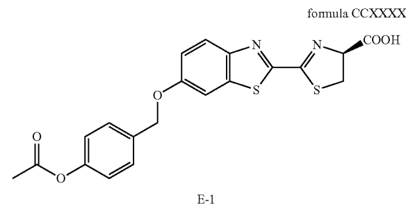
6(4-phosphoric acid benzylether) luciferin
