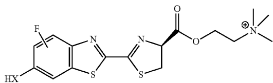
compound of formula XXXVIII
