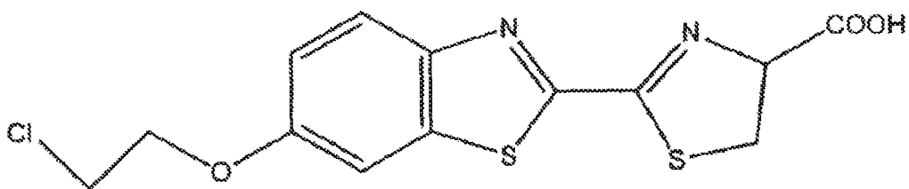
Luciferin 6' chloroethyl ether (Luciferin-CEE)
